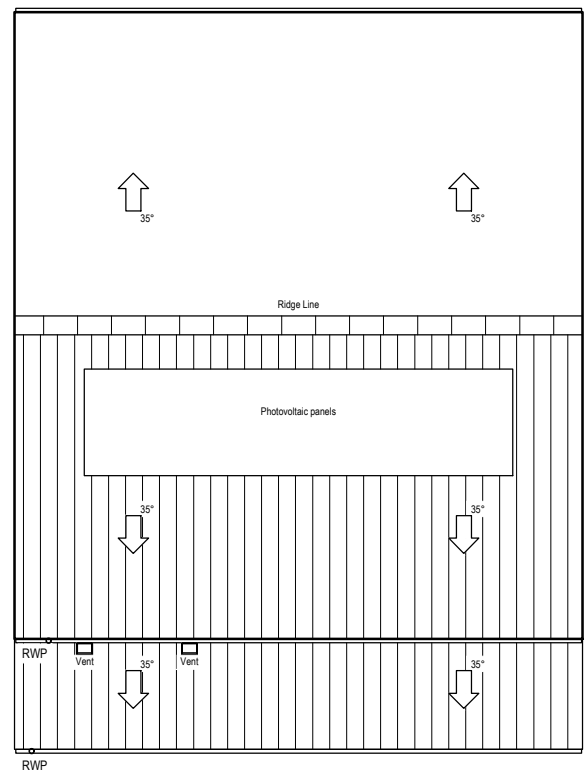
ROOF PLAN
