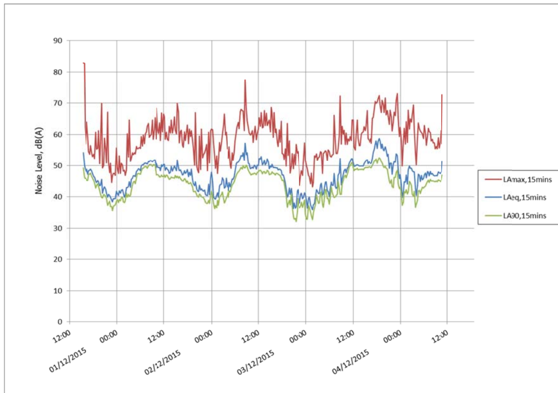
Chart 1: Background Sound Survey Time History
