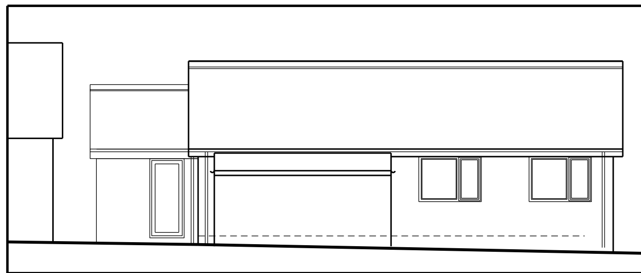
West Elevation - Proposed
