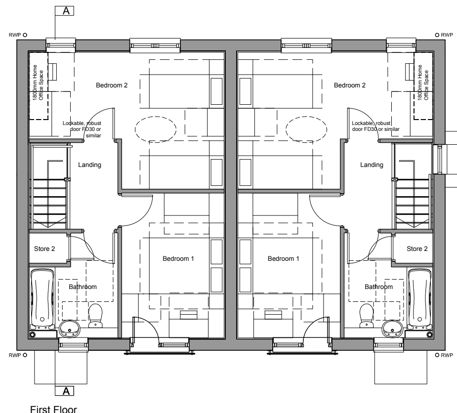
First Floor
