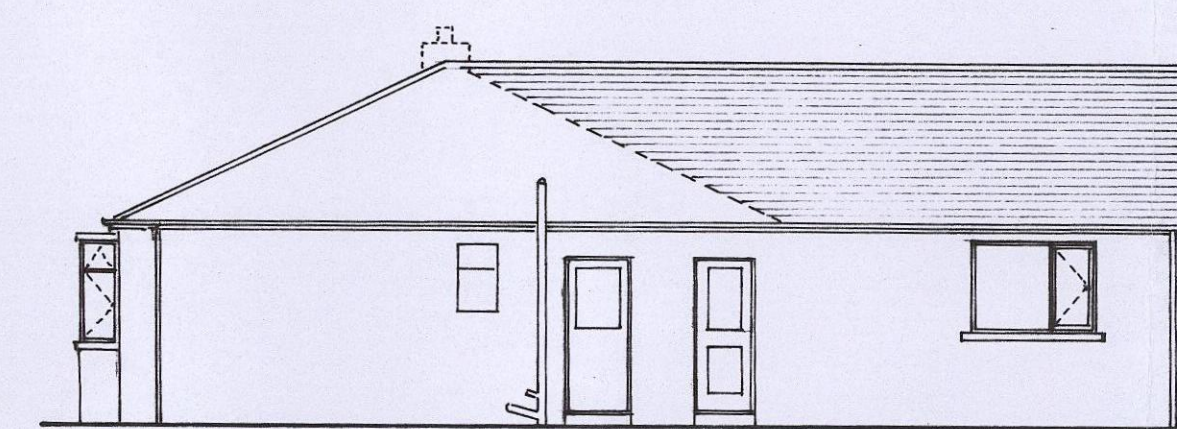
WEST ELEVATION
