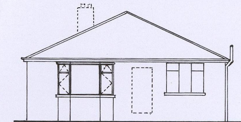
NORTH ELEVATION
