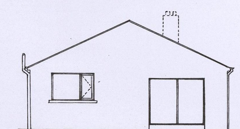
SOUTH ELEVATION
