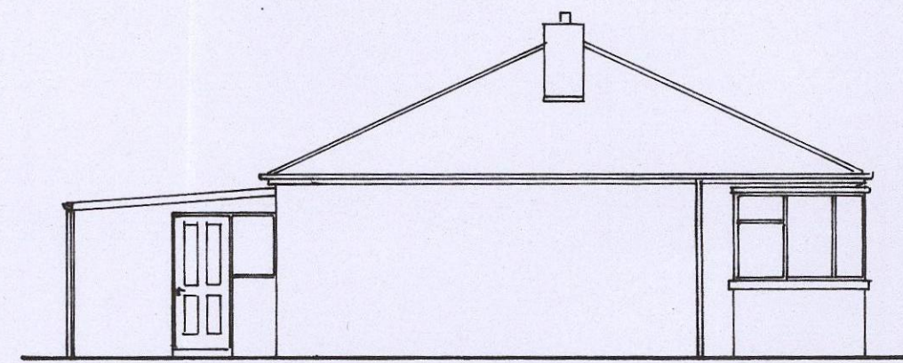
EAST ELEVATION
