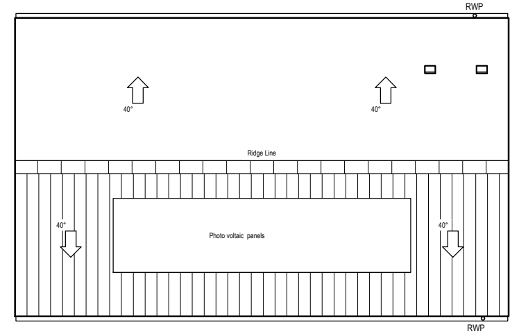
ROOF PLAN
