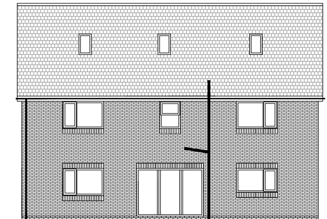
REAR ELEVATION
