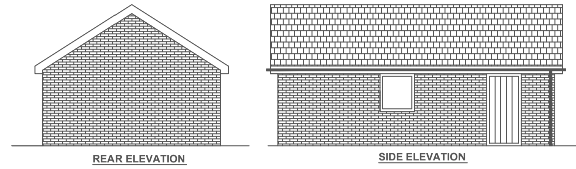
REAR ELEVATION
