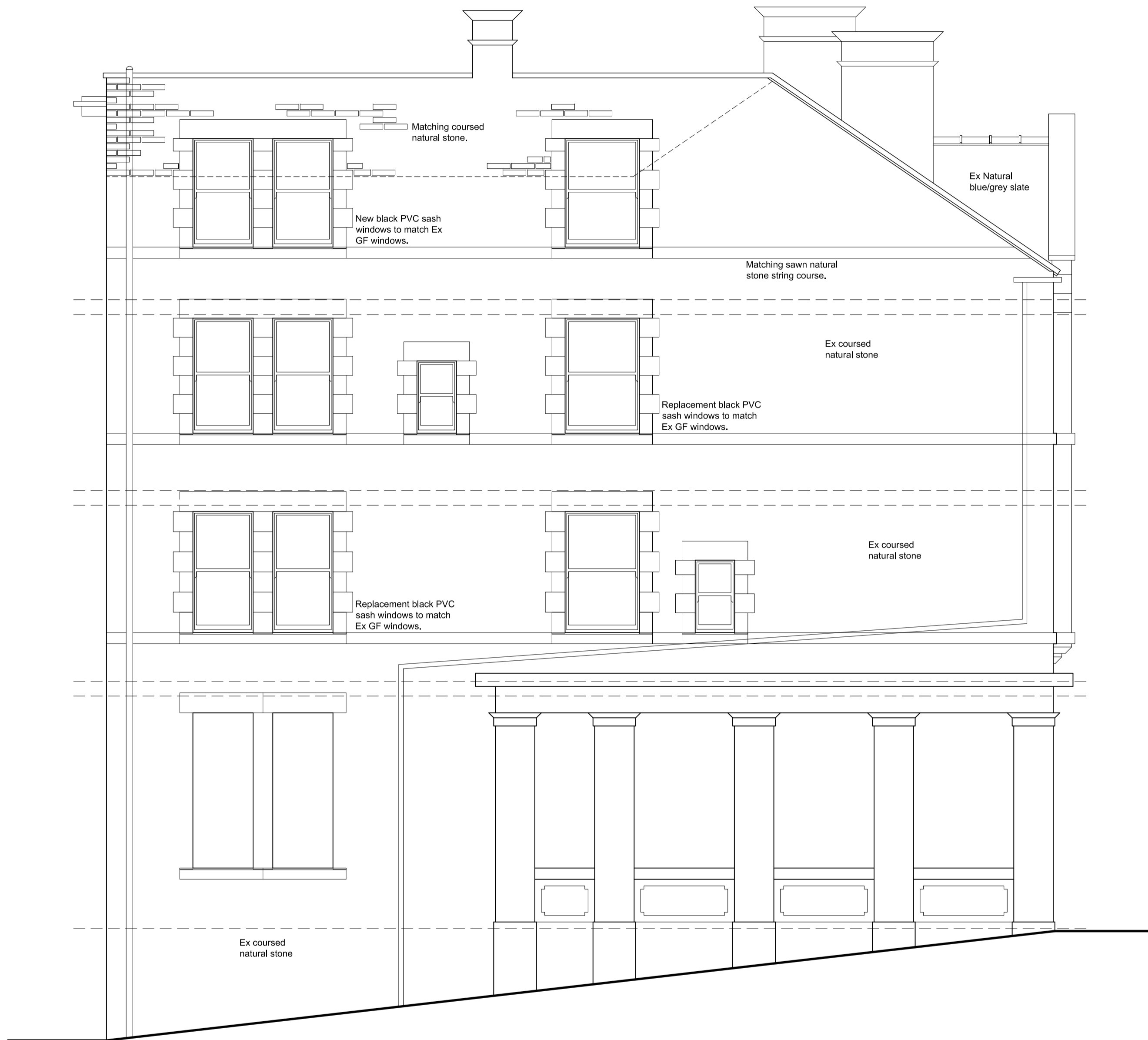
SIDE (NW) ELEVATION
