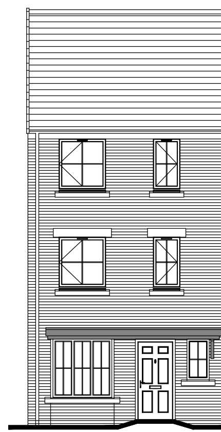
Front Elevation
