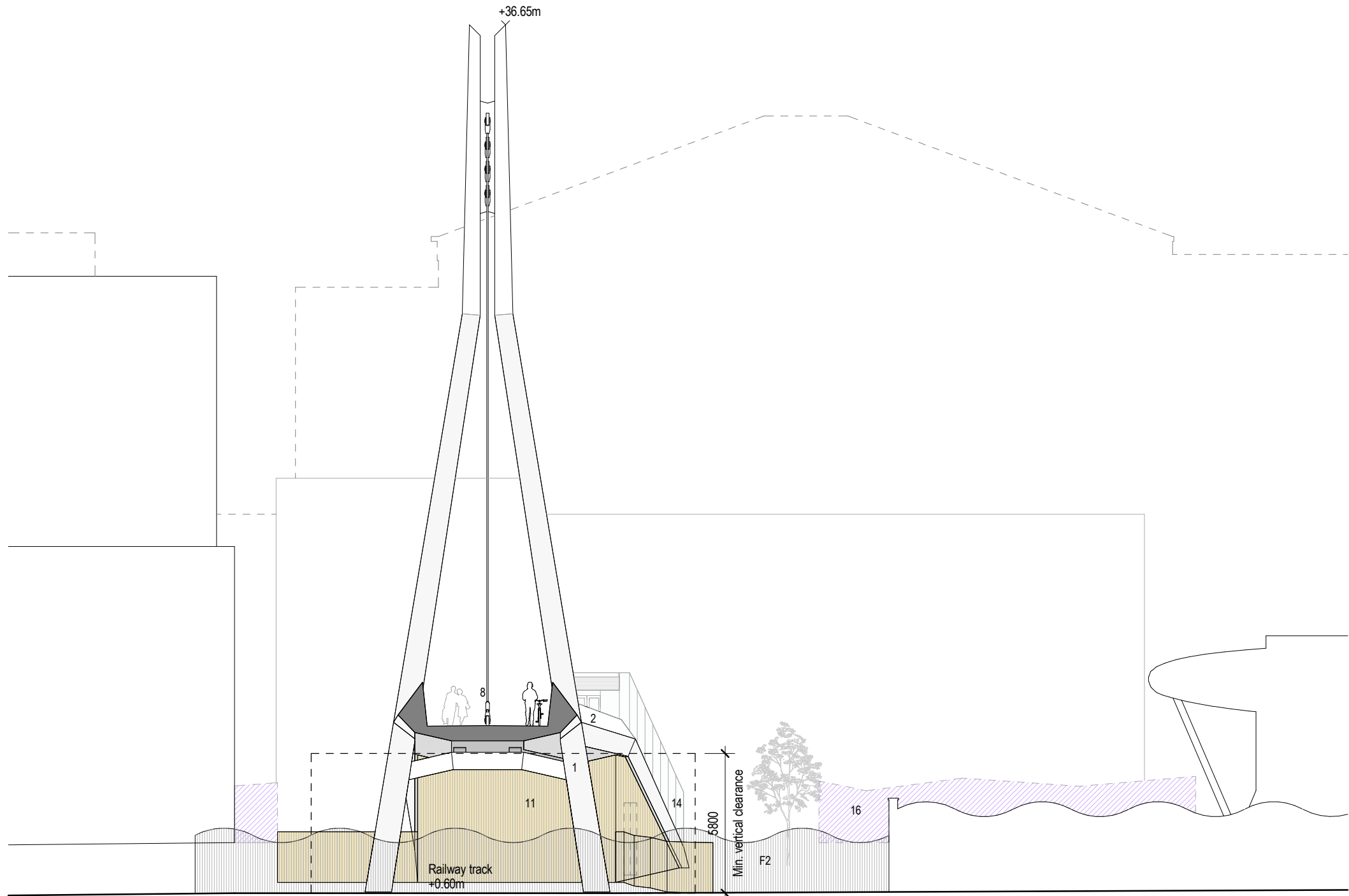
Proposed Section D - D 1:200
