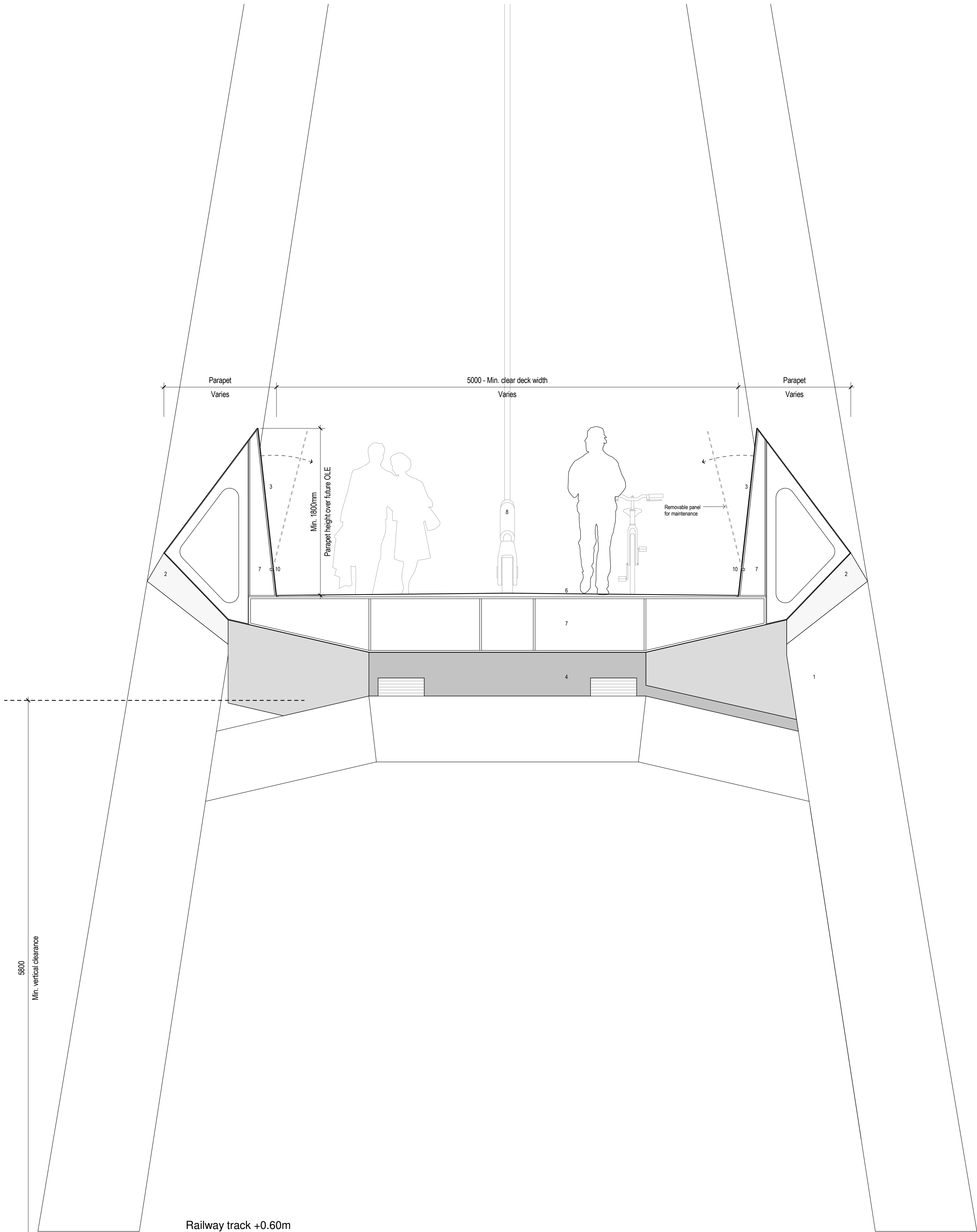
Deck Cross Section 1:25
