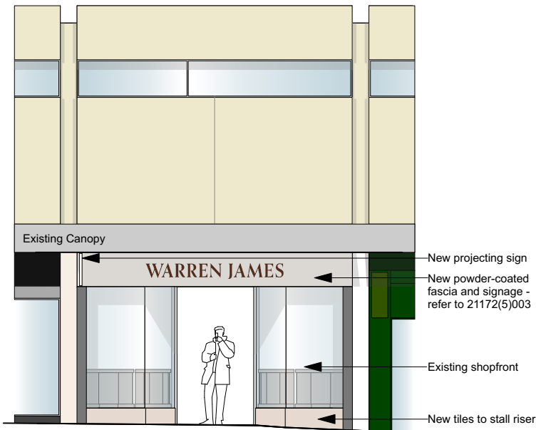
Proposed Elevation Scale 1:100
