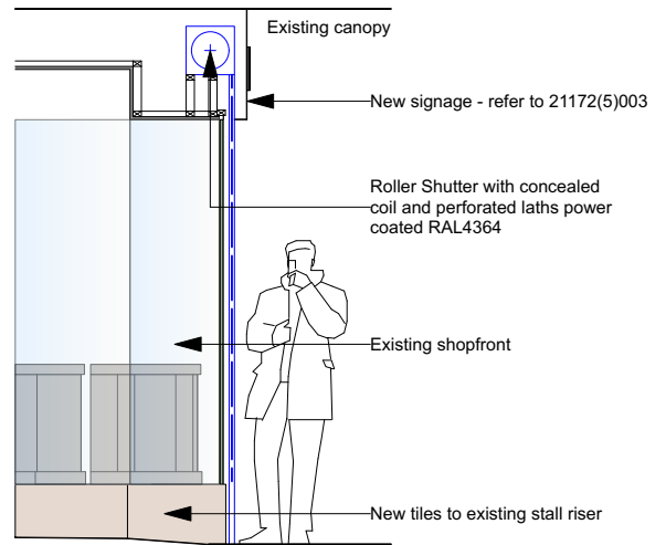
Proposed Section Scale 1:50
