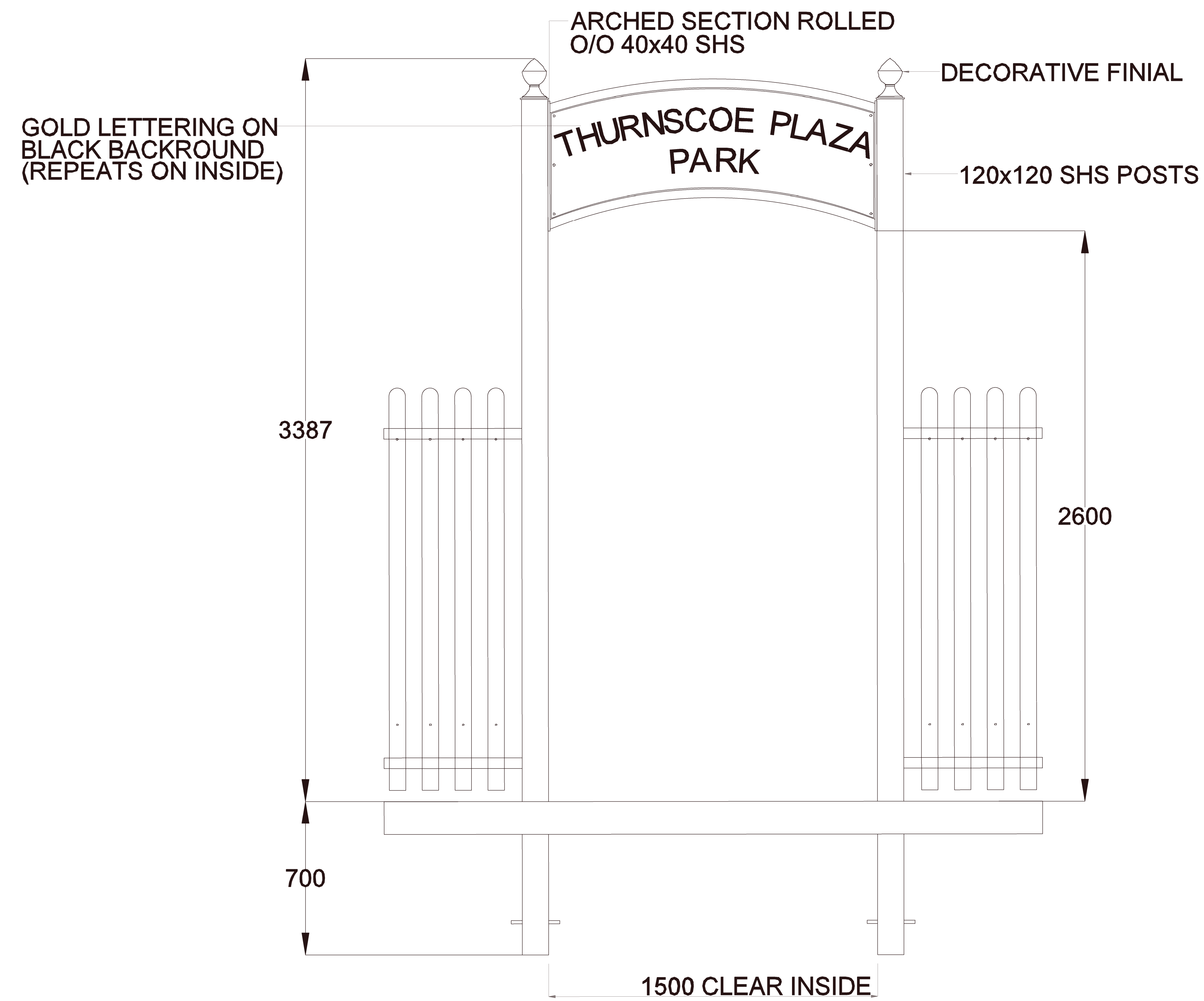
ELEVATION FROM OUTSIDE
