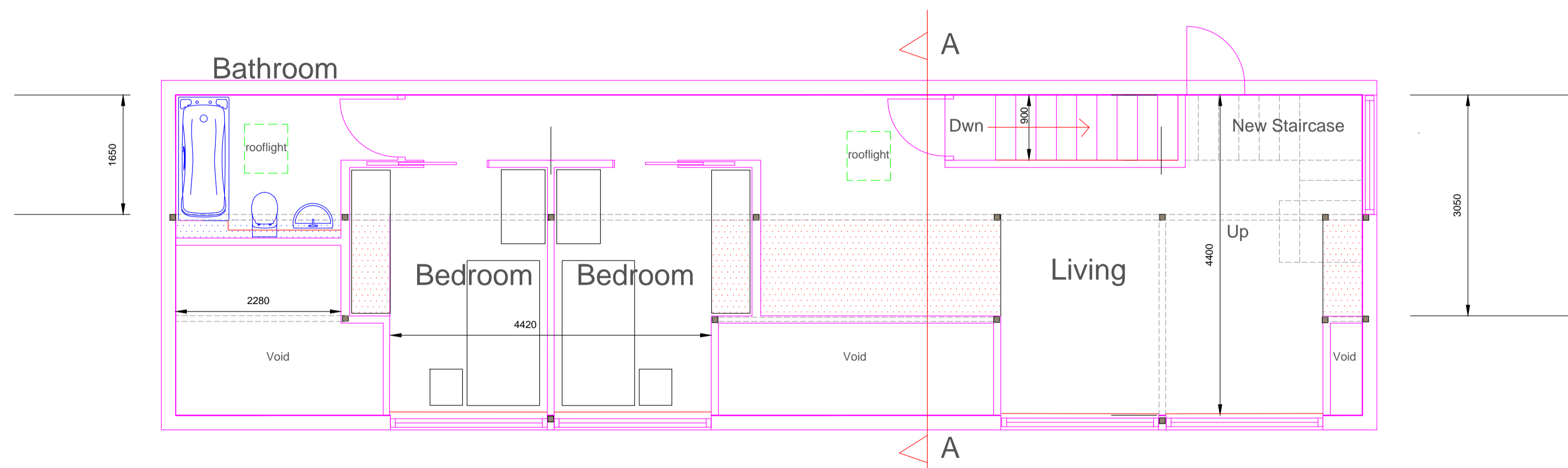
Proposed New Roof Extension
