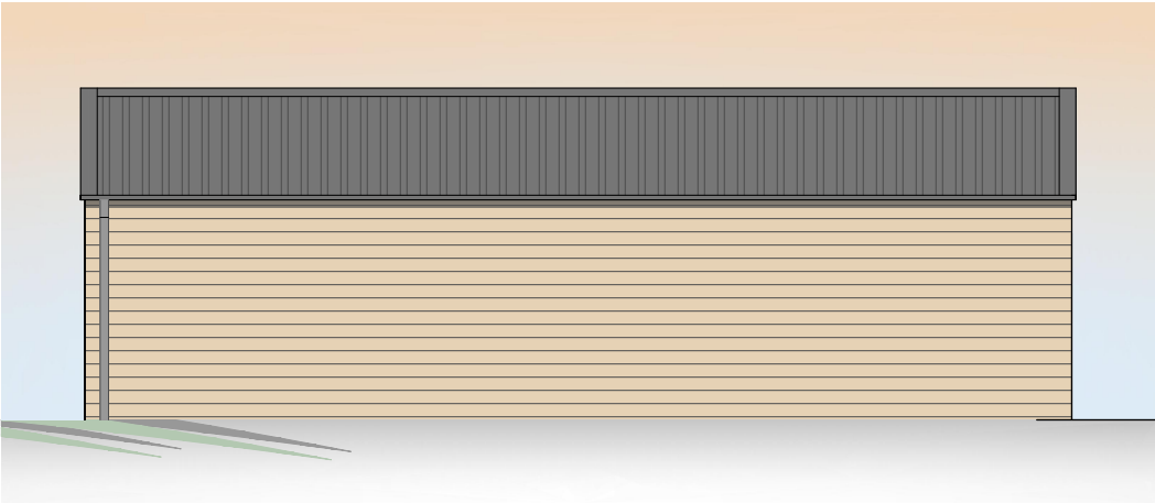
Proposed South Facing Elevation
