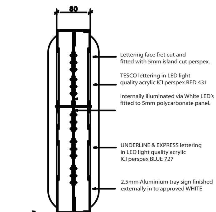
A - Internal section of sign
