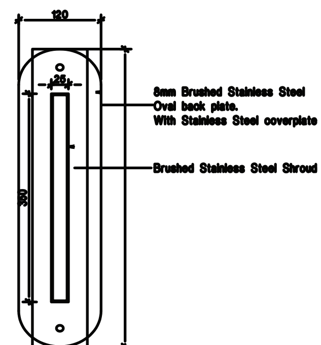
B - Showing outer casing of projecting sign
