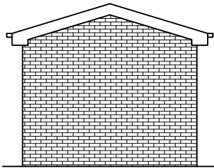
PROPOSED REAR ELEVATION SCALE 1:100 AT A3
