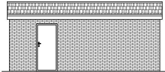
PROPOSED SIDE ELEVATION SCALE 1:100 AT A3
