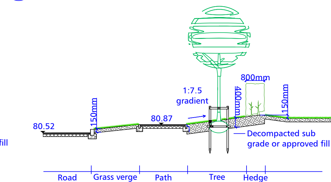
Section D 1:100 NORTH GAWBER ENTRANCE - ENTRANCE ROAD
