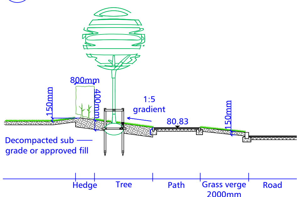
Section G 1:100 NORTH GAWBER ENTRANCE - ENTRANCE ROAD
