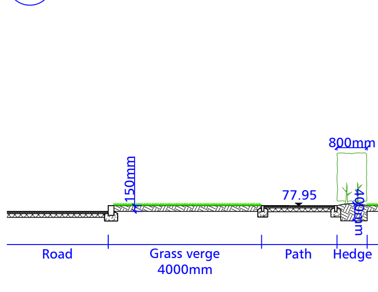
Section L 1:100 NORTH GAWBER ENTRANCE - CARR GREEN LANE
