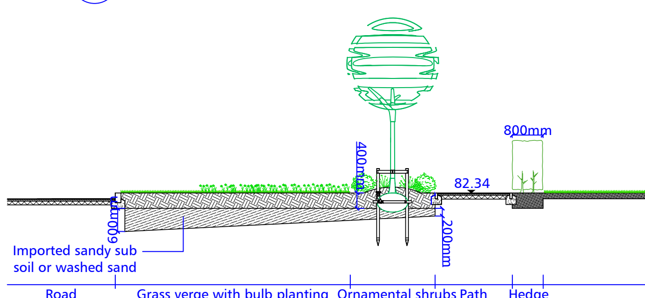
Section D 1:100 NORTH GAWBER ENTRANCE - ENTRANCE ROAD
