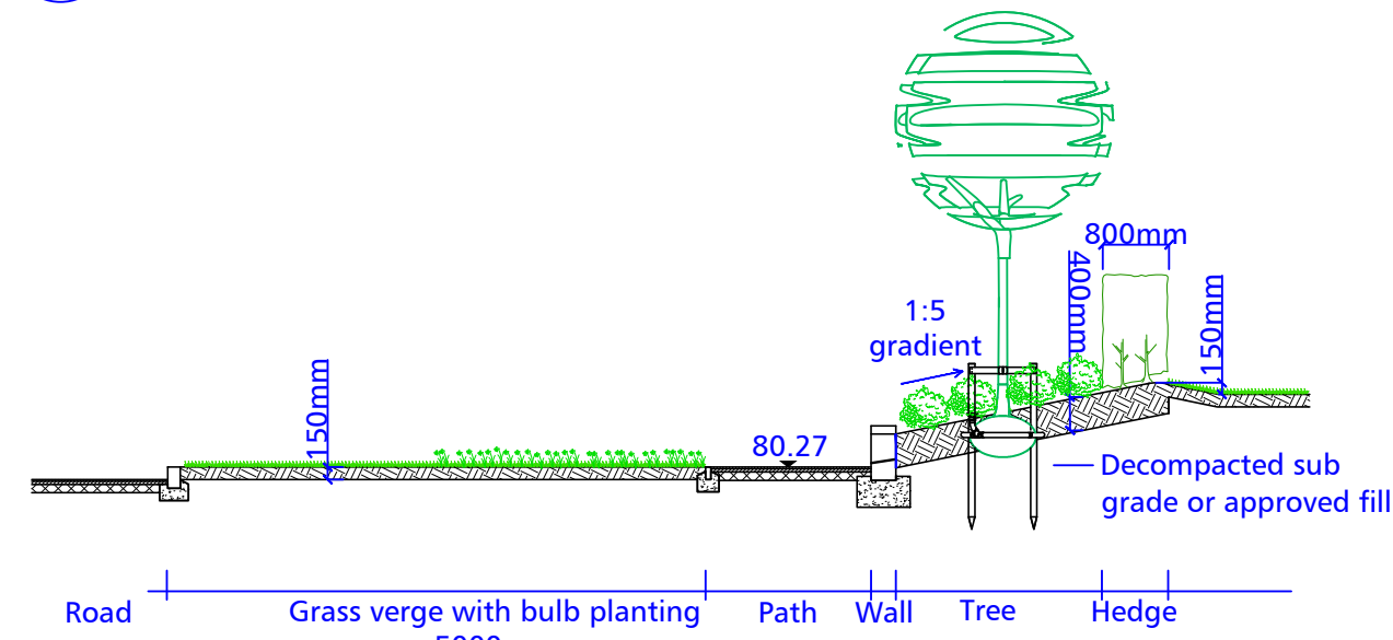
Section C 1:100 NORTH GAWBER ENTRANCE - CARR GREEN LANE
