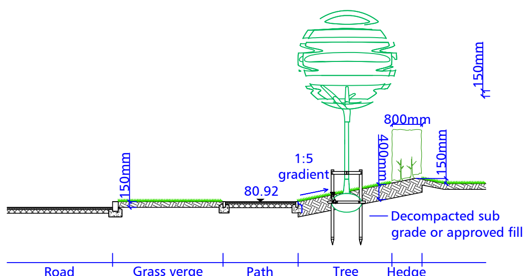
Section B 1:100 NORTH GAWBER ENTRANCE - CARR GREEN LANE
