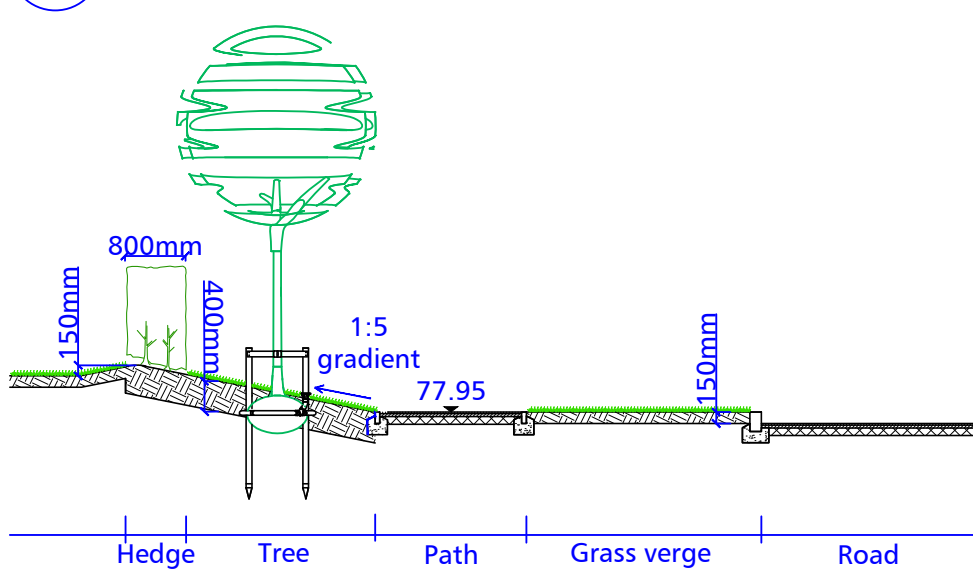
Section K 1:100 NORTH GAWBER ENTRANCE - CARR GREEN LANE
