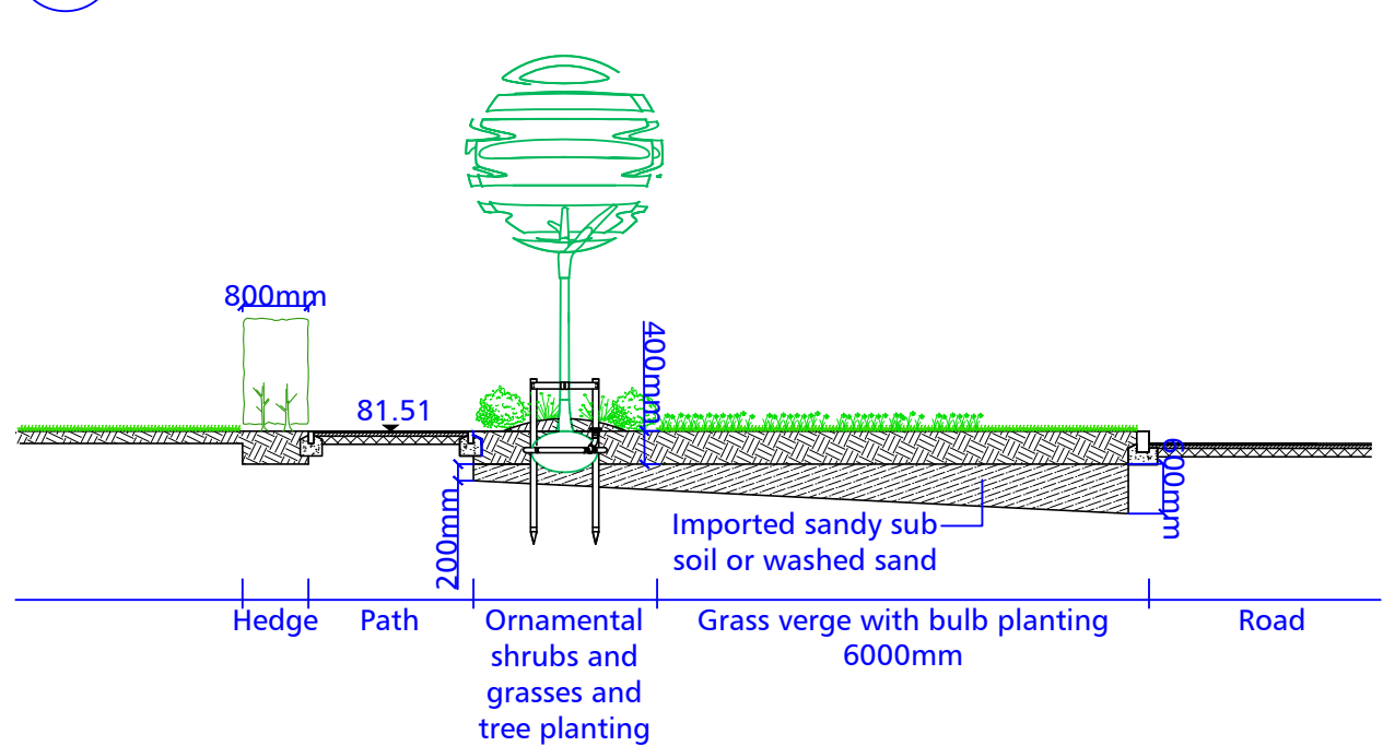
Section H 1:100 NORTH GAWBER ENTRANCE - ENTRANCE ROAD
