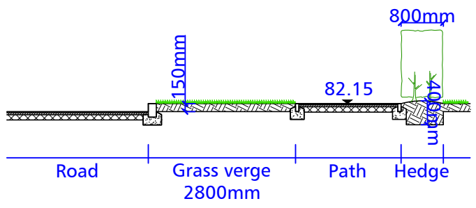
Section A 1:100 NORTH GAWBER ENTRANCE - CARR GREEN LANE
