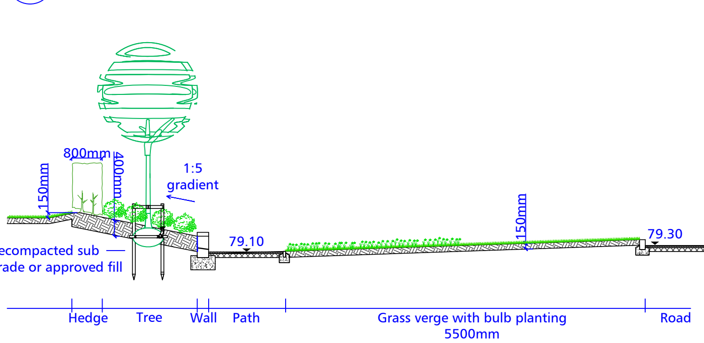
Section J 1:100 NORTH GAWBER ENTRANCE - CARR GREEN LANE
