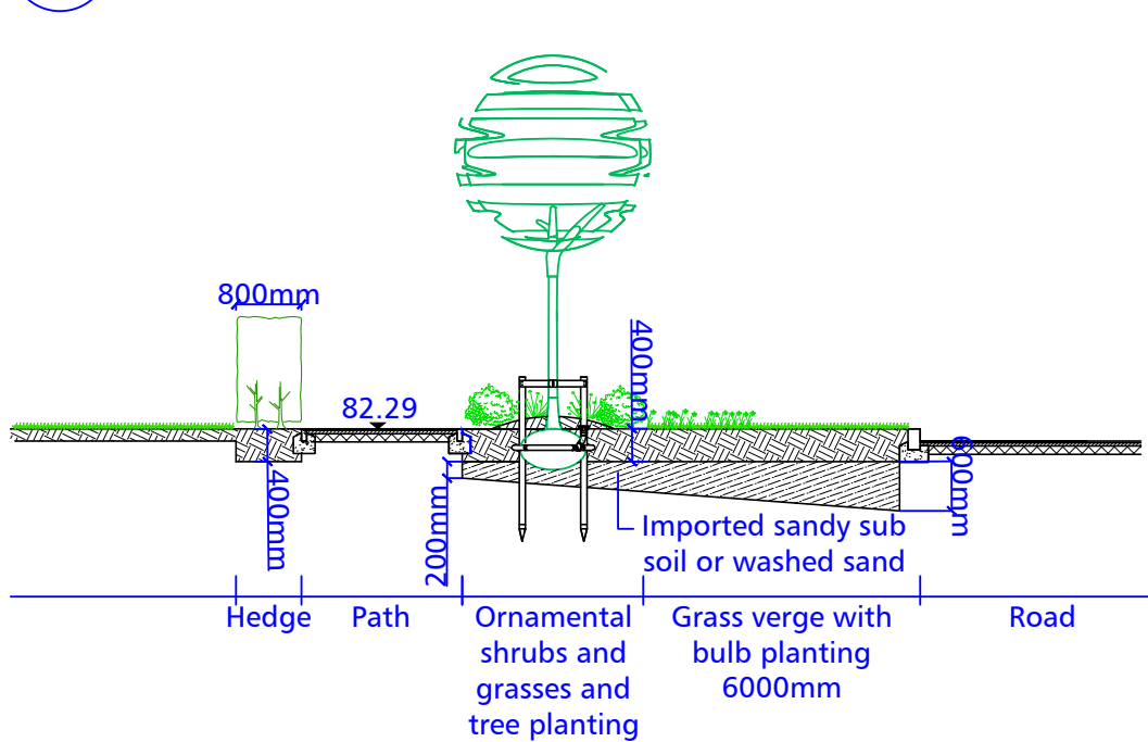
Section G 1:100 NORTH GAWBER ENTRANCE - ENTRANCE ROAD
