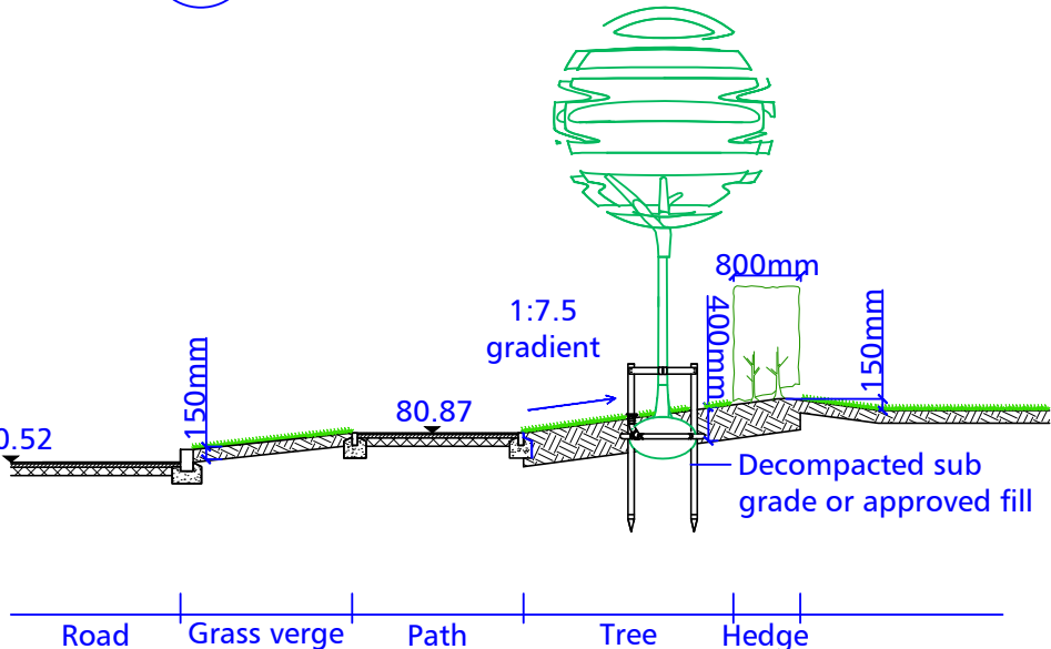
Section C 1:100 NORTH GAWBER ENTRANCE - CARR GREEN LANE
