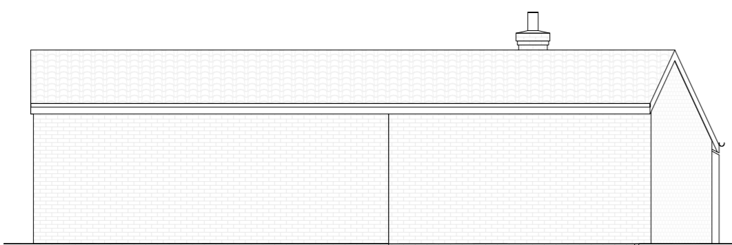
4 Proposed Side Elevation 1 : 100
