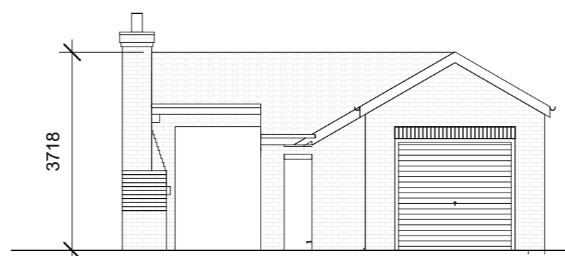
2 Proposed Front Elevation 1 : 100
