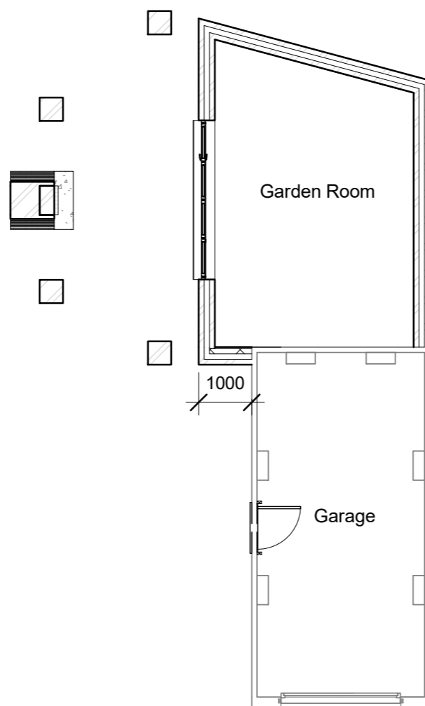
6 Proposed Ground Floor Plan 1 : 100
