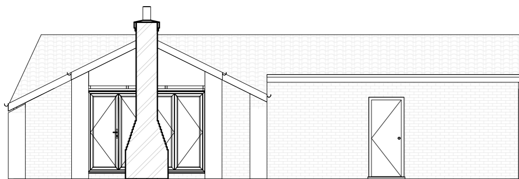
5 Proposed Side Elevation 1 1 : 100
