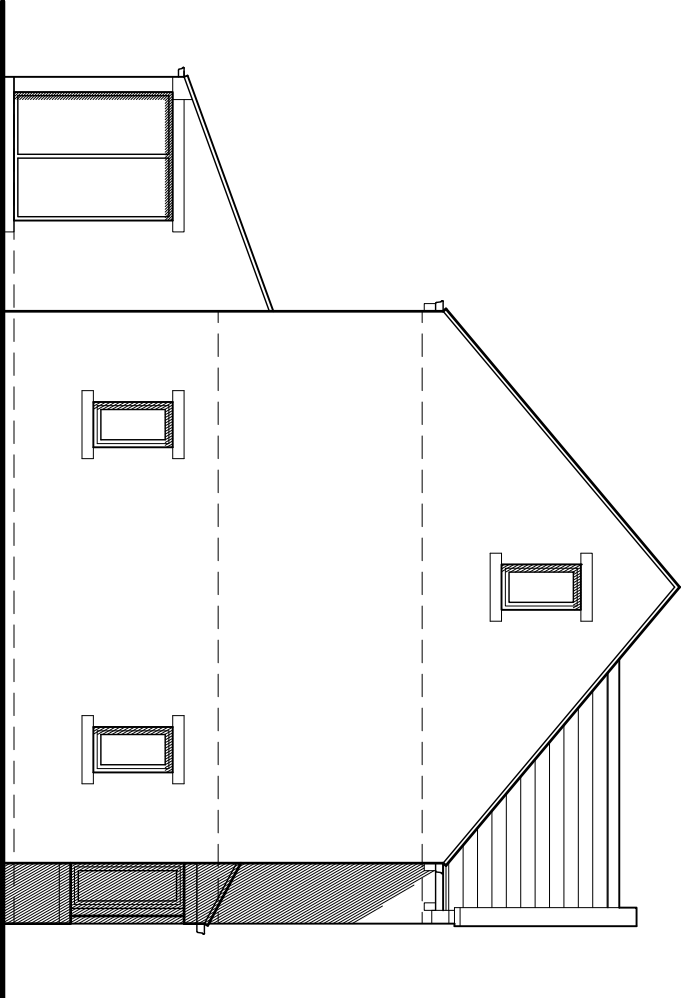
Side Elevation
