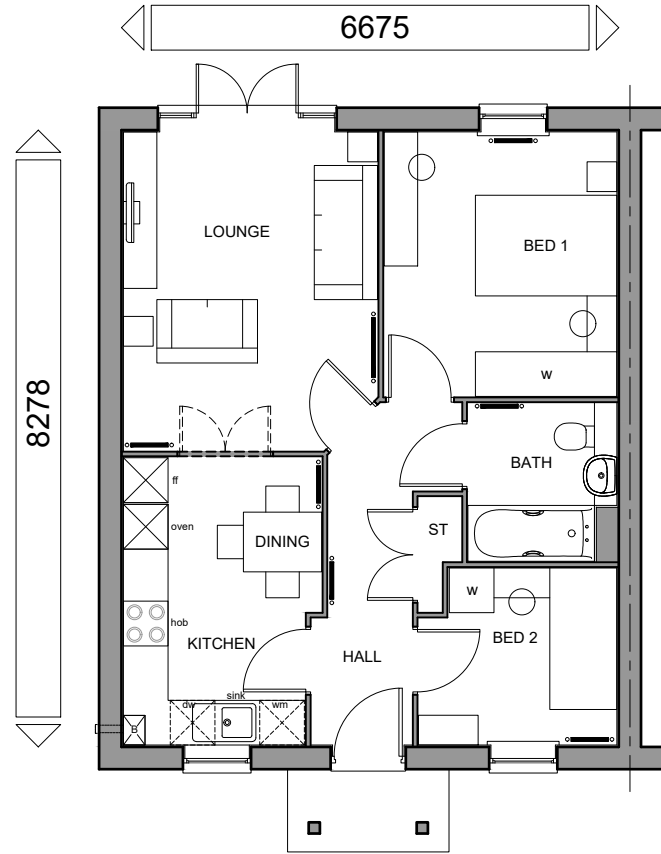
FLOOR PLAN
