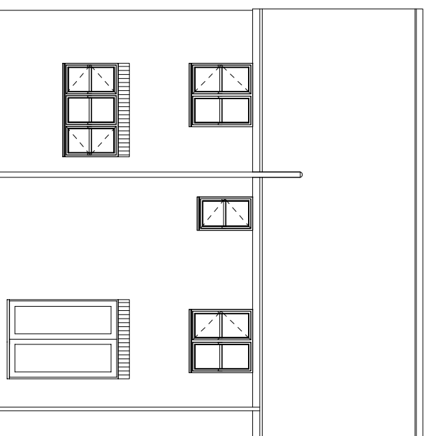
REAR ELEVATION
