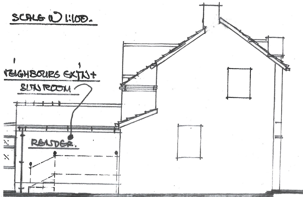
EXISTING SIDE VIEW.
