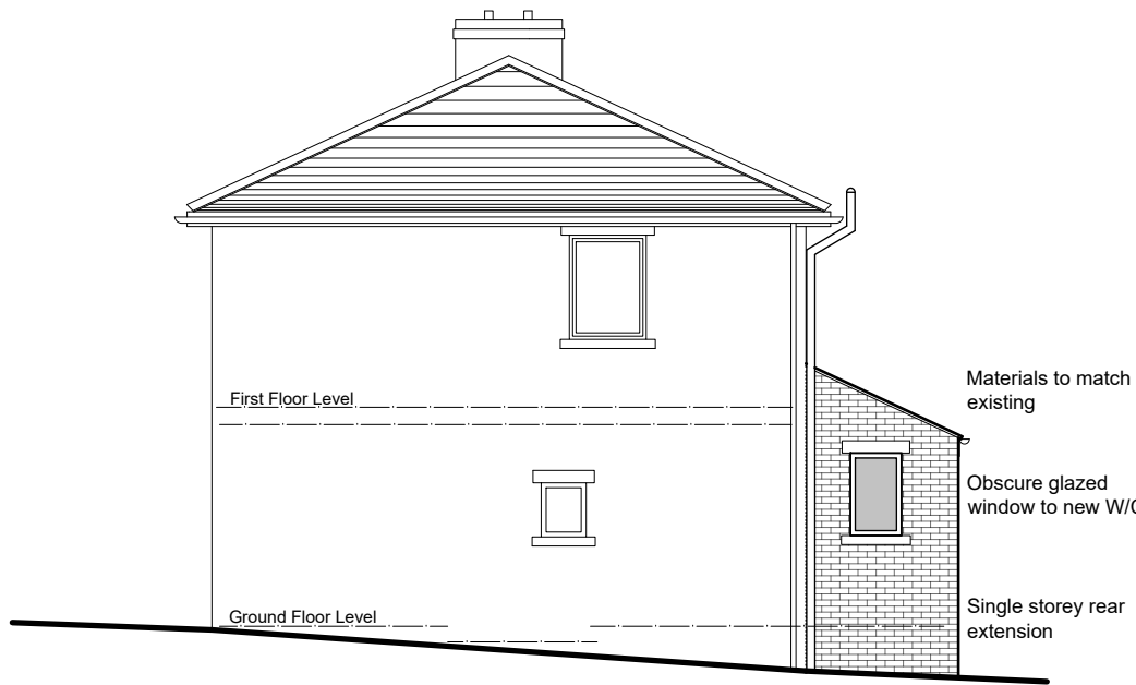
East Elevation (side)
