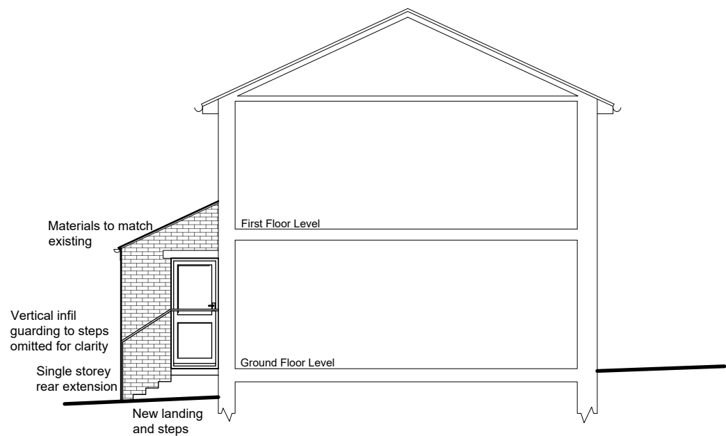
West Sectional Elevation (side (Party Wall))
