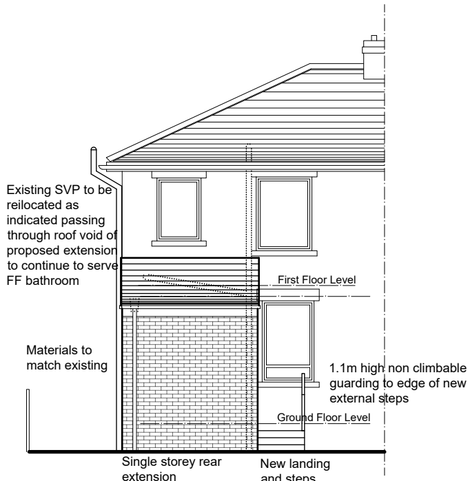
North Elevation (rear)
