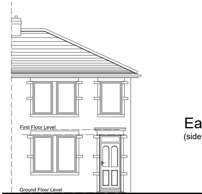
South Elevation (front)
