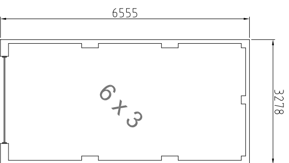
Floor Plan 1:100
