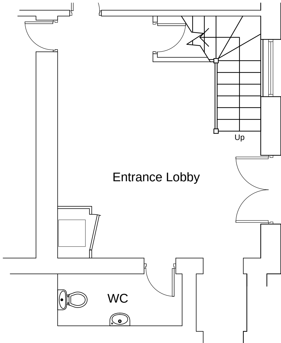
01 Existing Ground Floor Lobby 1:50
