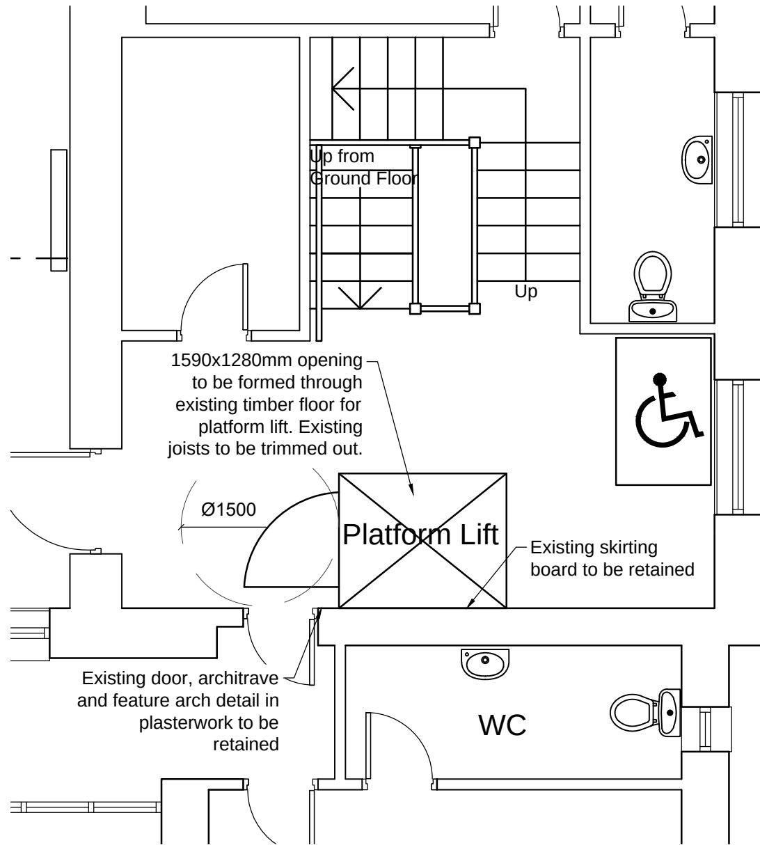
04 Proposed First Floor Lobby 1:50
