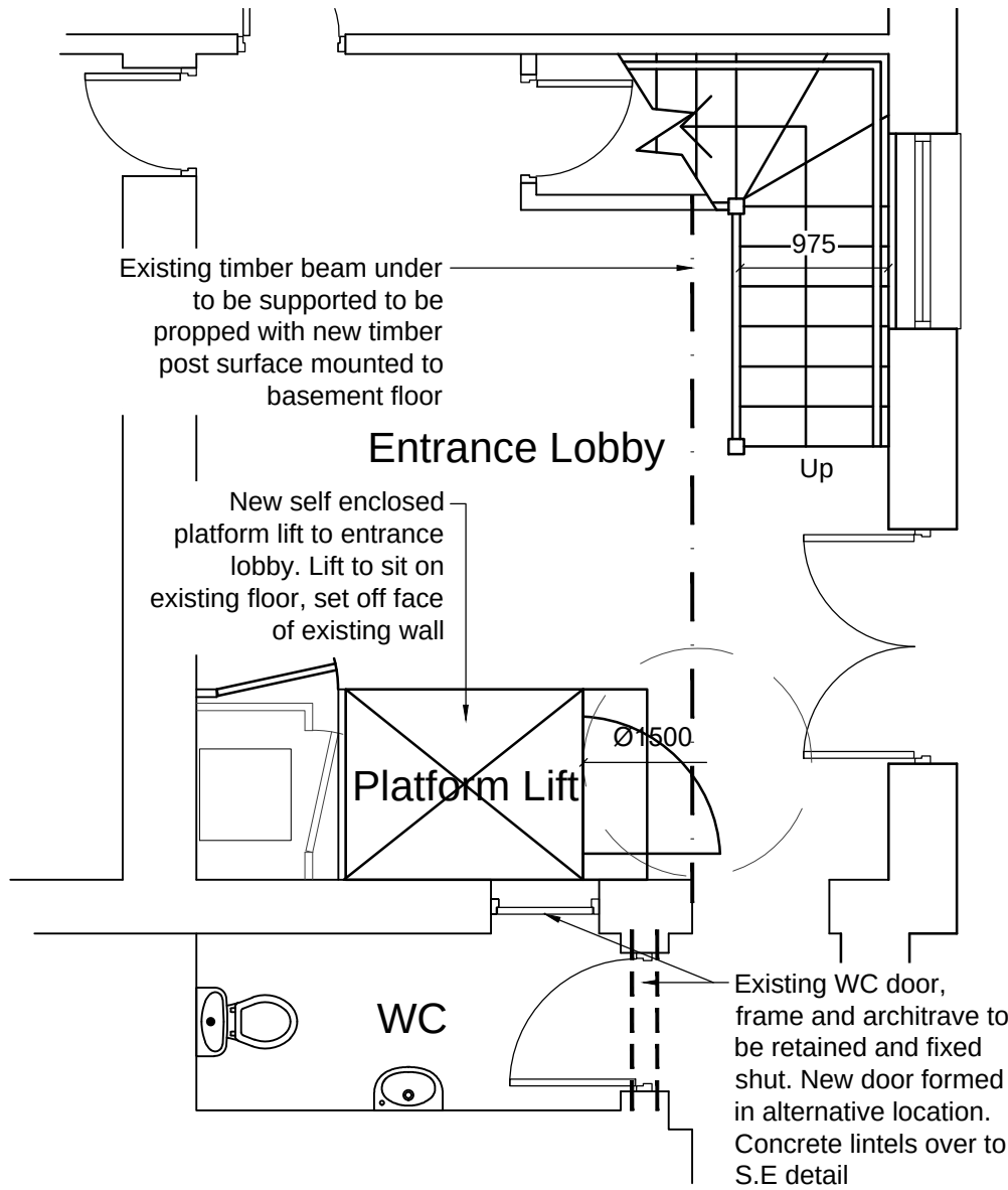
03 Proposed Ground Floor Lobby 1:50
