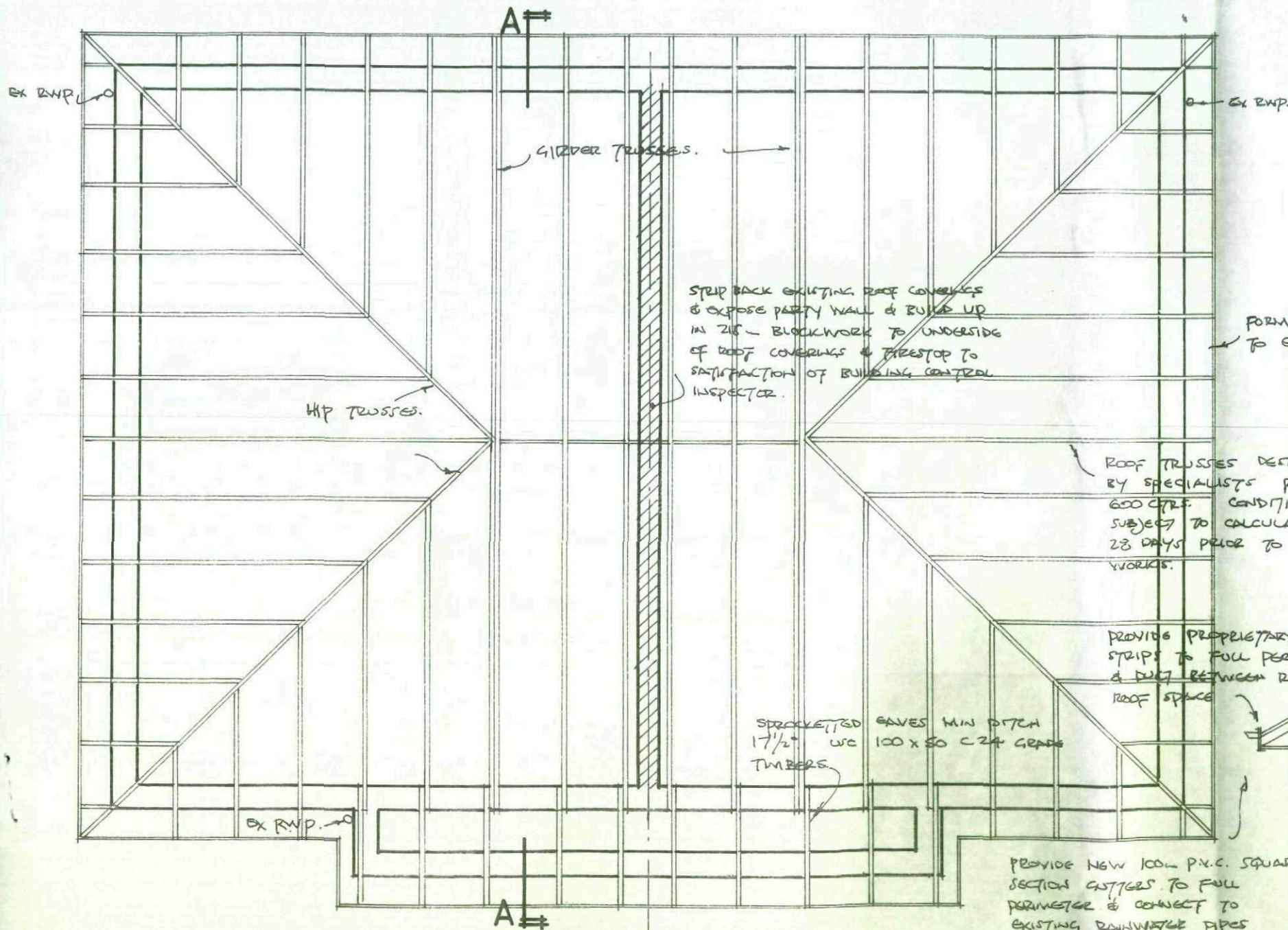
PROPOSED ROOF PLAN SUPERIMPOSED ON EXISTING WALL LAYOUT (1:50)
