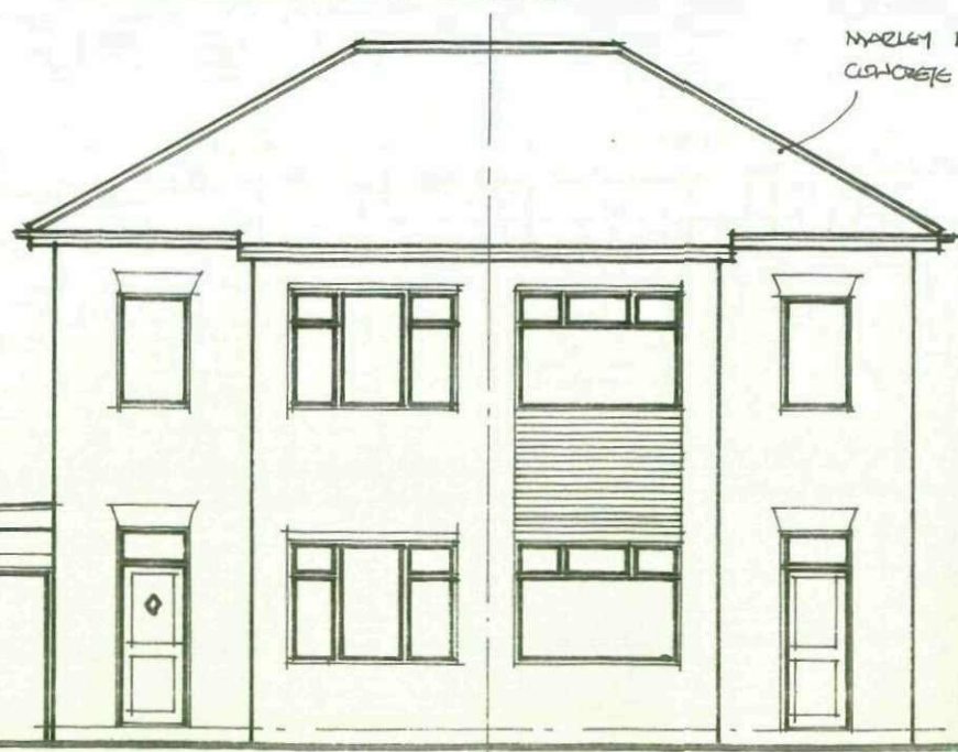
PROP. FRONT ELEVATIONS (1:100)
