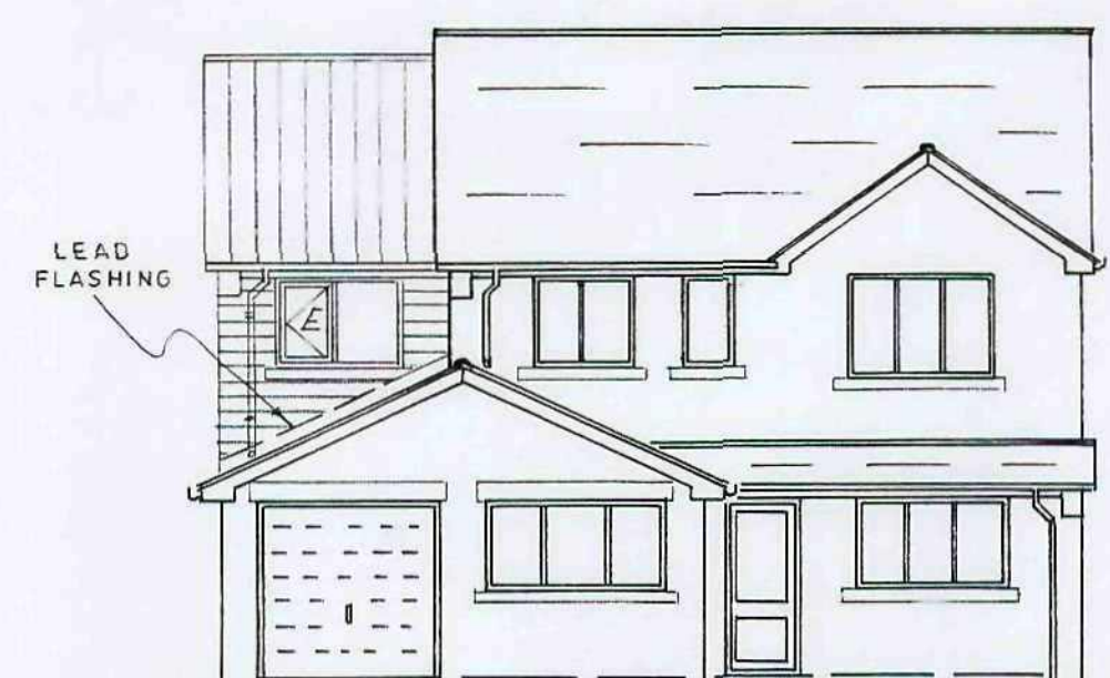
PROPOSED FRONT
