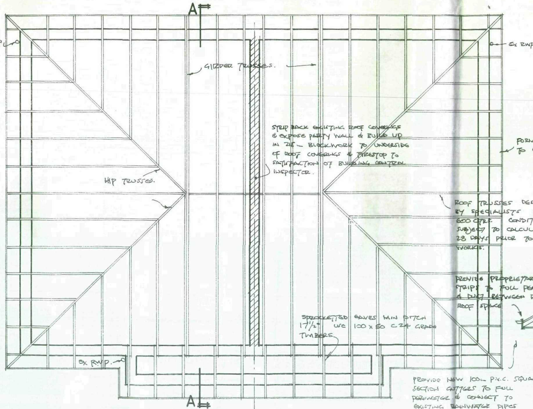
PROPOSED ROOF PLAN SUPERIMPOSED ON EXISTING WALL LAYOUT (1:50)
