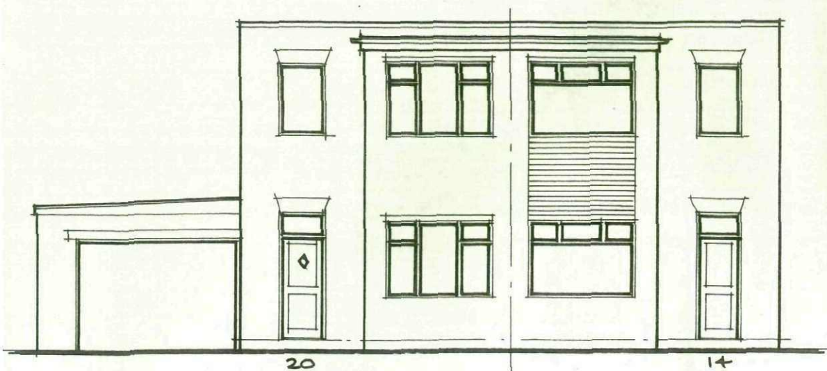
EX. FRONT ELEVATIONS (1:100)
