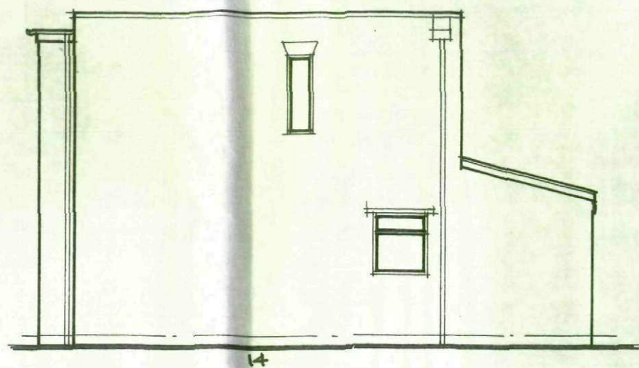
EX. SIDE ELEVATION (1:100)
