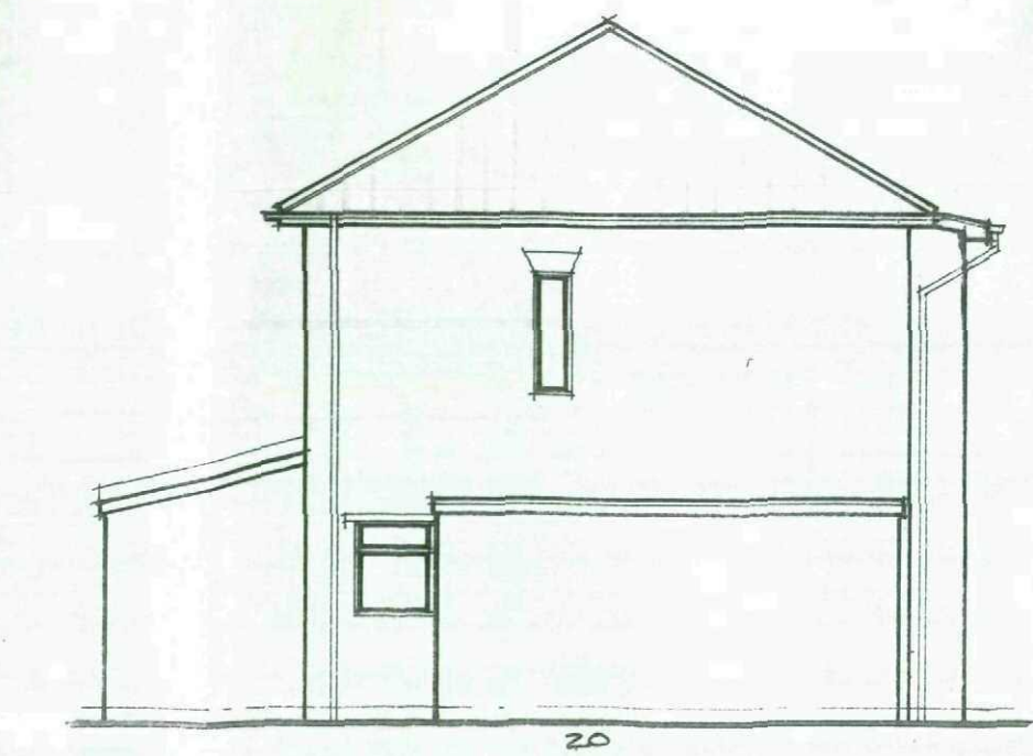
PROP. SIDE ELEVATION (1:100)
