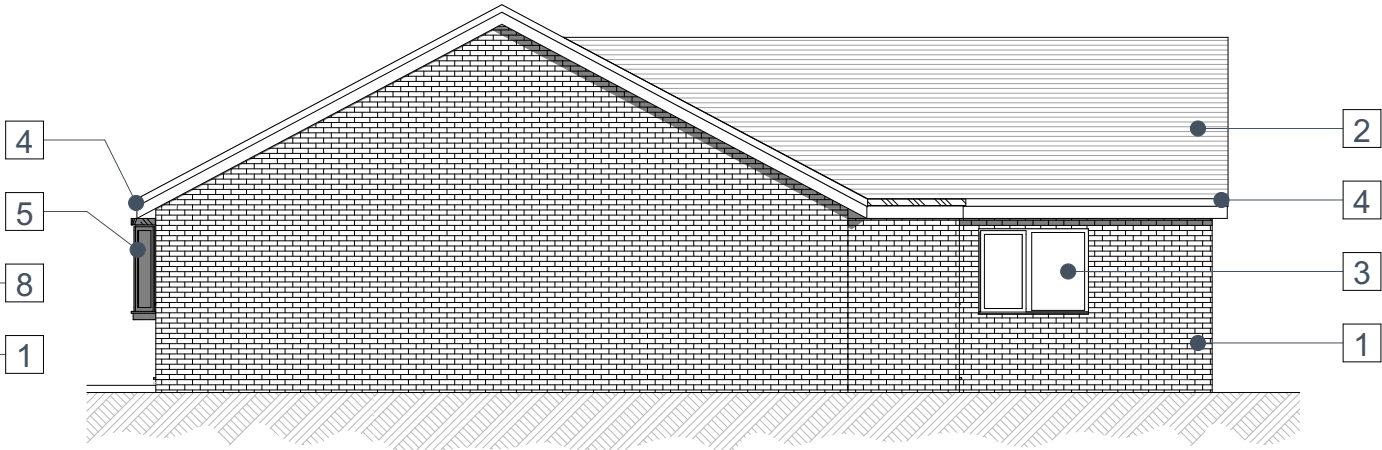
E02 E02 Existing Rear Elevation 1:100
