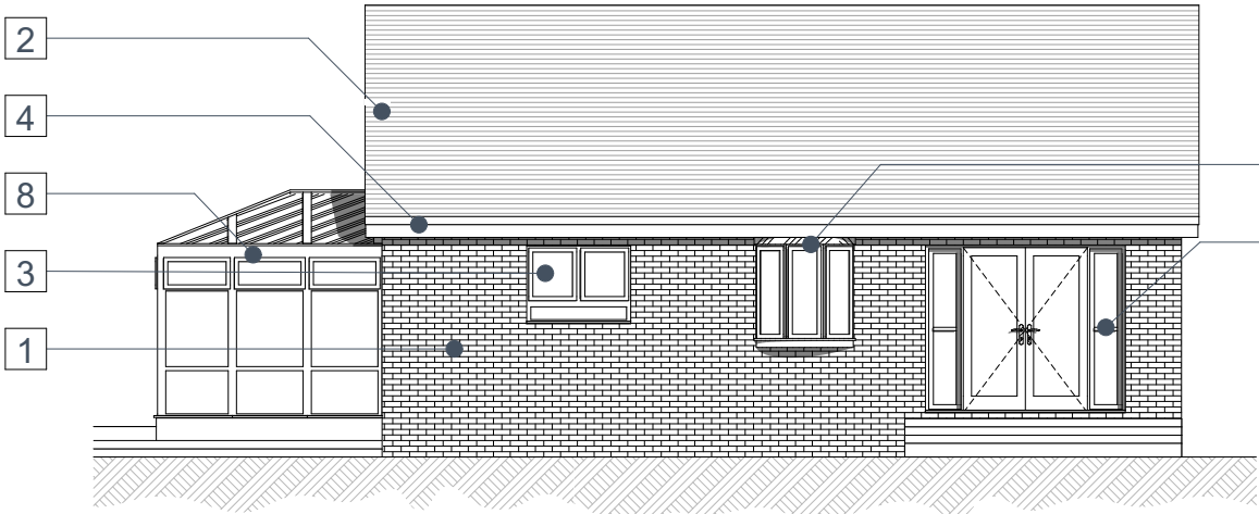
E03 E03 Existing Side Elevation 1:100
