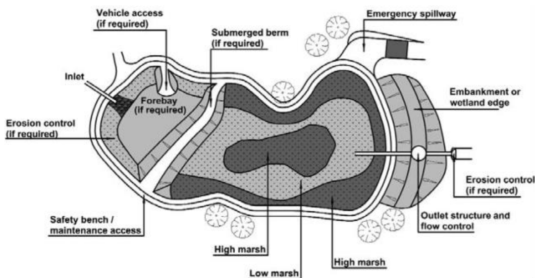
Figure 13(a) – A Typical Wetland Arrangement (Plan View)
