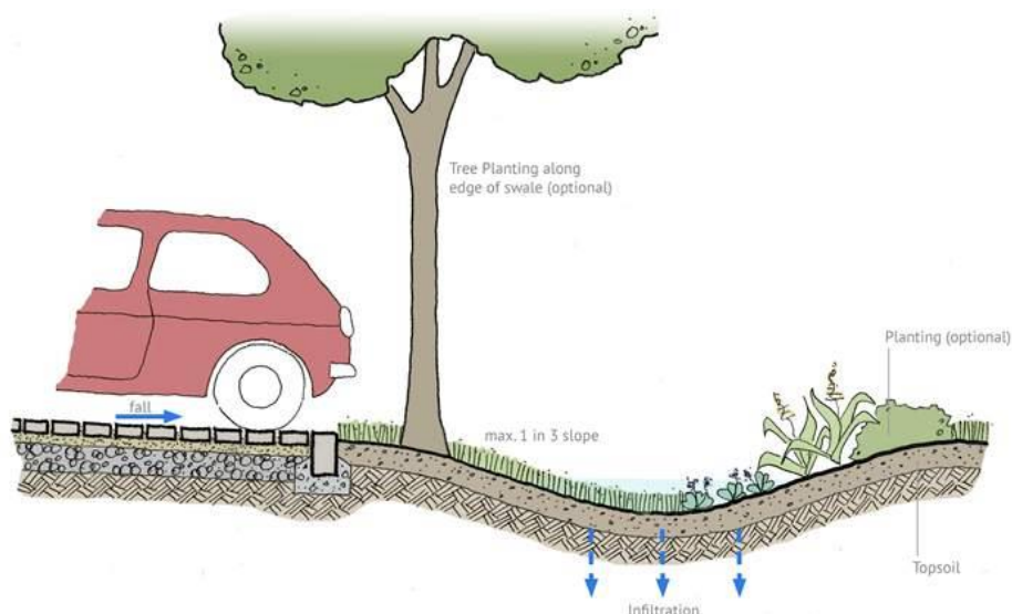
Figure 6 - A Typical Swale Construction
