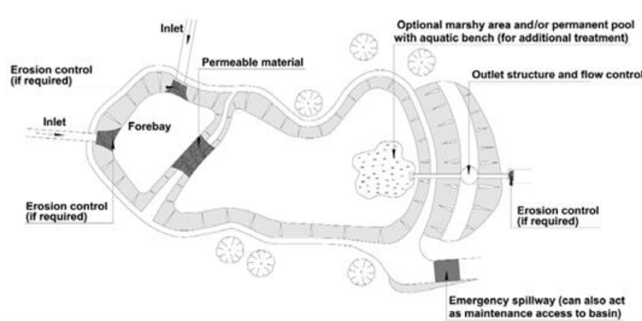
Figure 11(a) – A Typical Detention Basin (Plan View)
