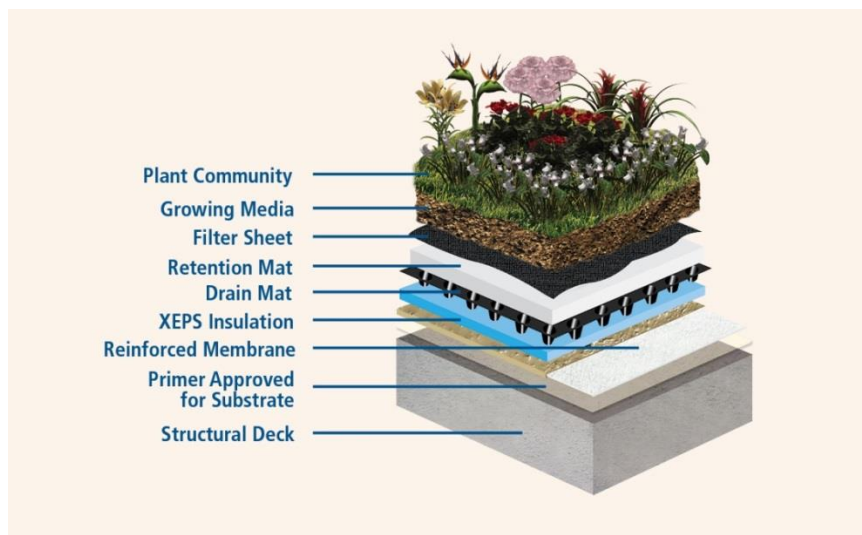
Figure 3 - A Typical Green-Roof Construction
