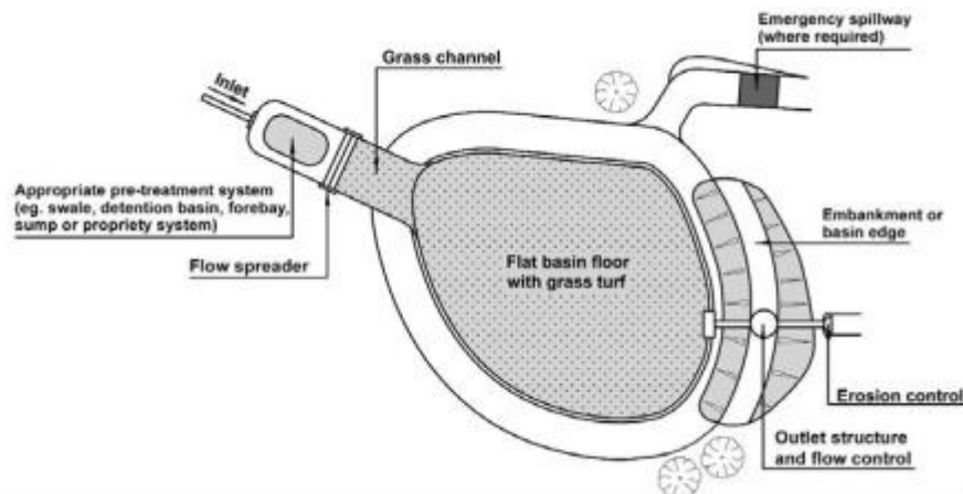
Figure 10(a) – A Typical Infiltration Basin (Plan View)
