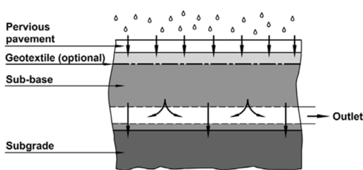
Figure 9(b) - Pervious Pavement System Types: Type B – Partial Infiltration
