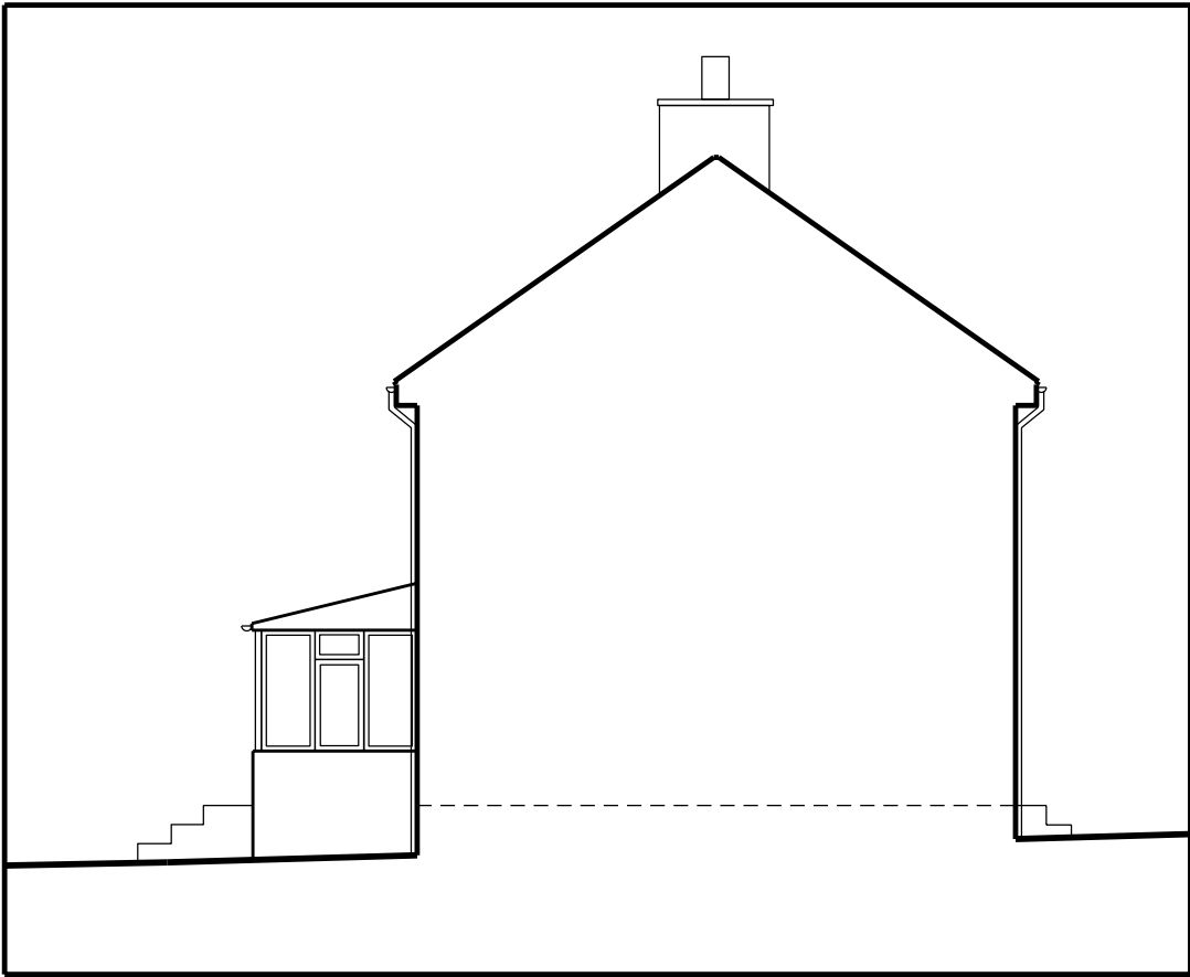
West Elevation - Existing
