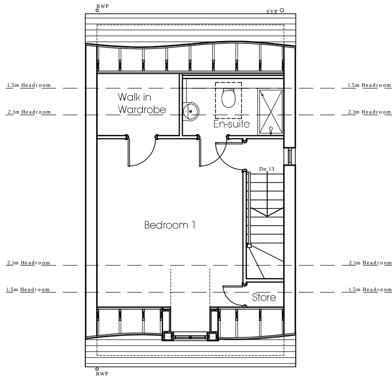
Second Floor
