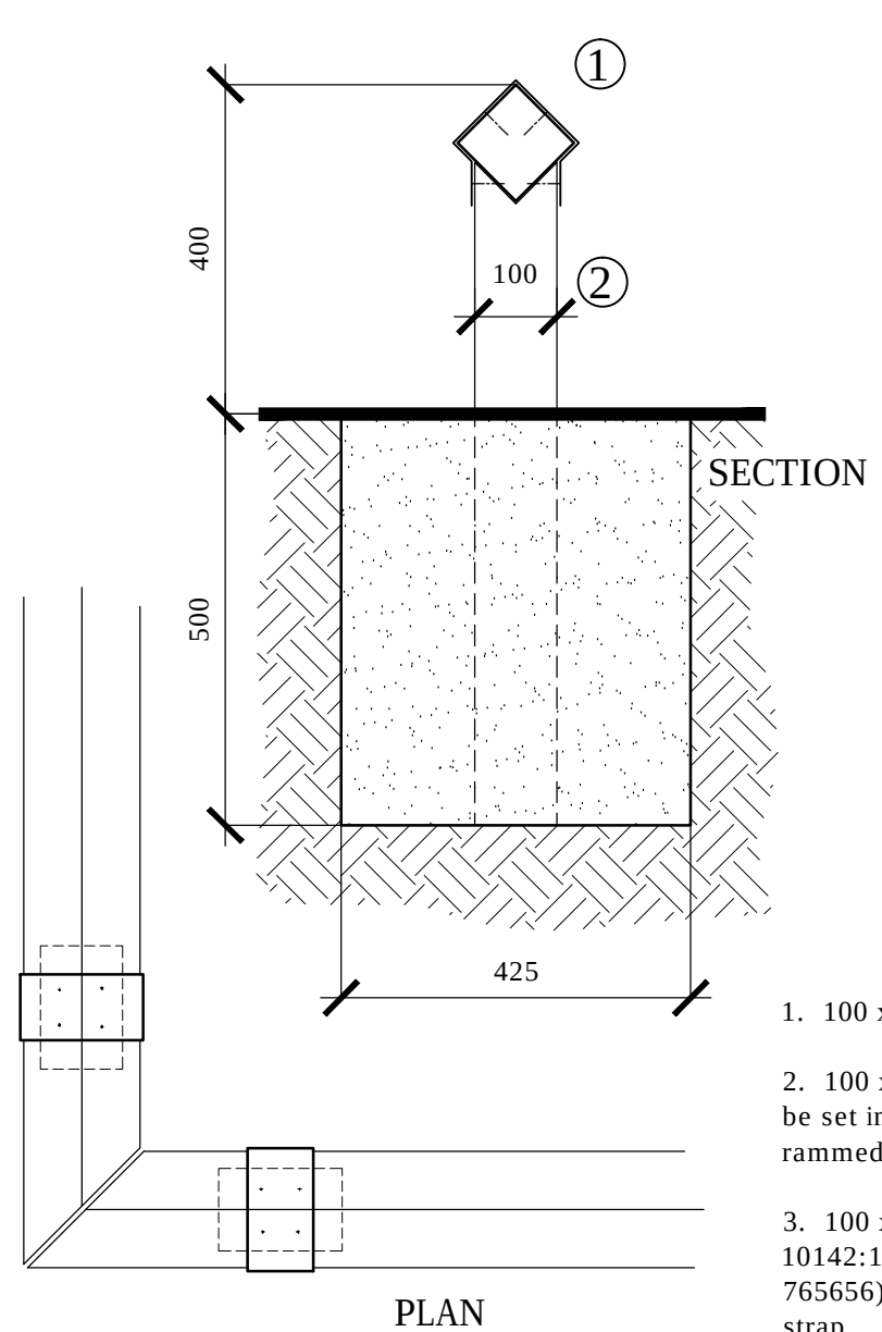
Fence Type A Knee Rail
