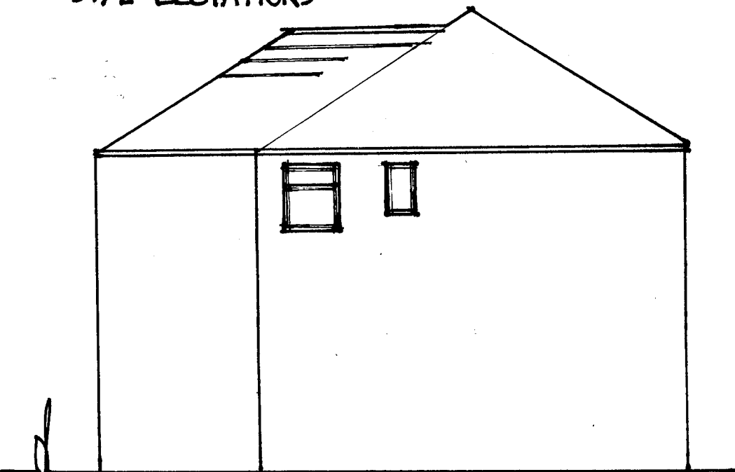
SIDE ELEVATIONS
