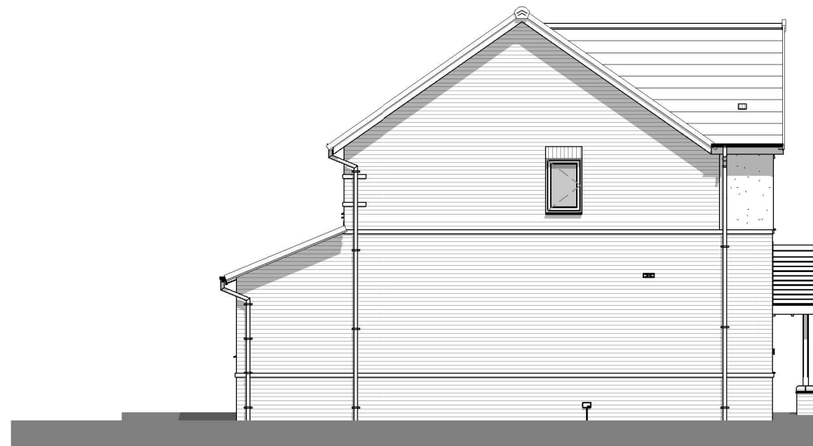
Left Side Elevation. 1 : 100
