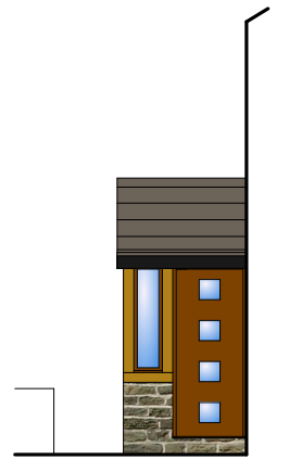
proposed side of porch elevation
