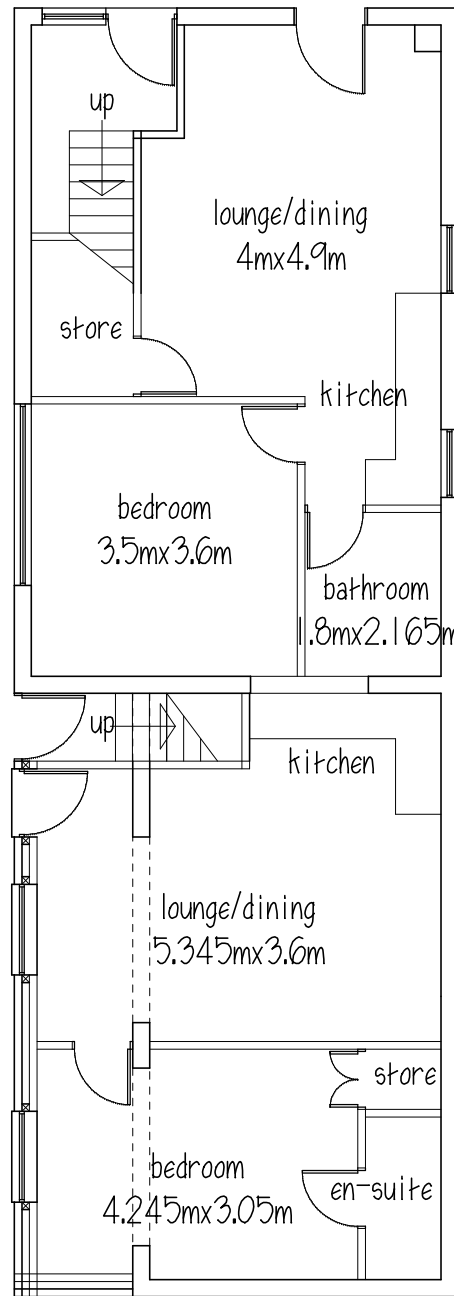
GROUND FLOOR
