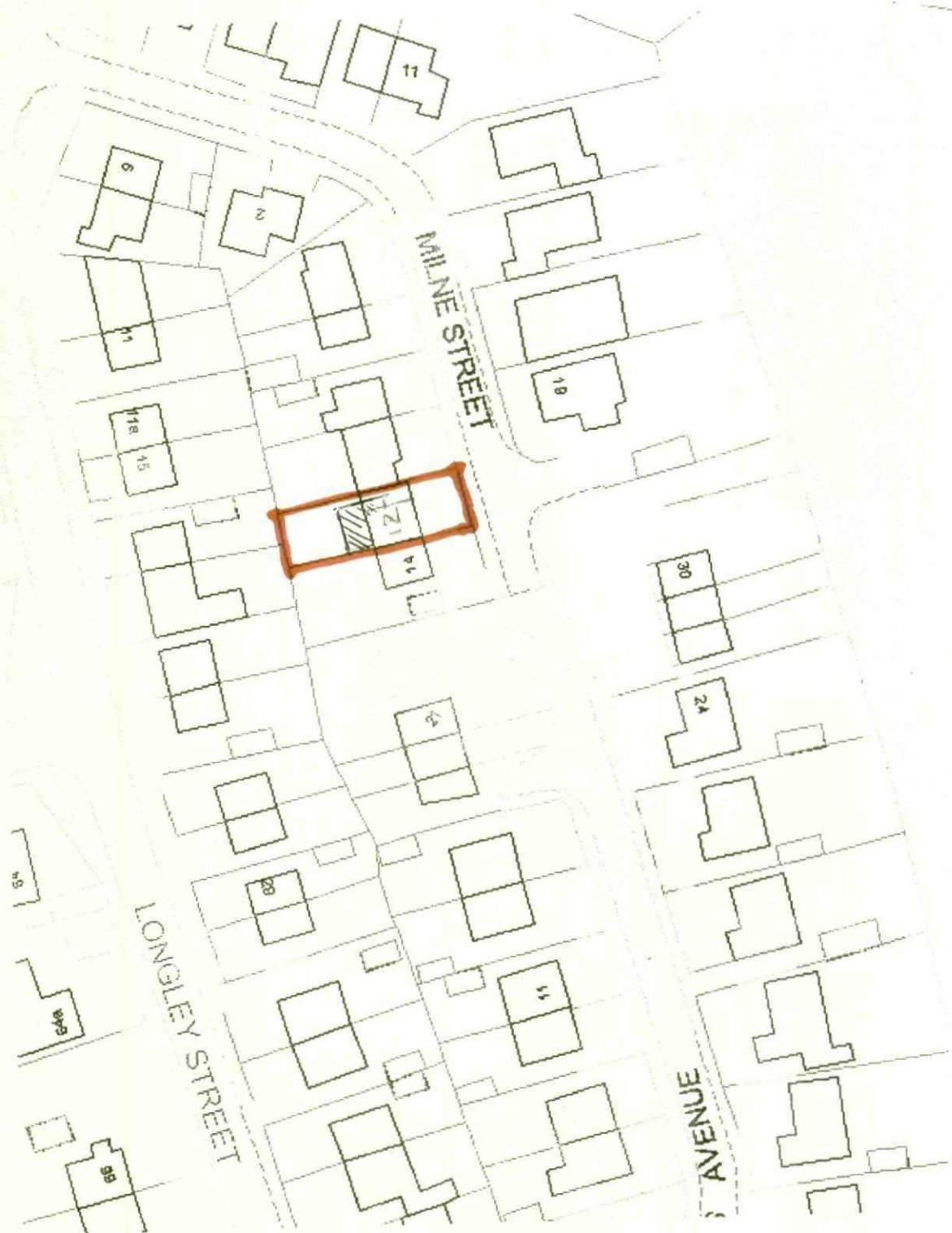
LOCATION PLAN 1:1000
