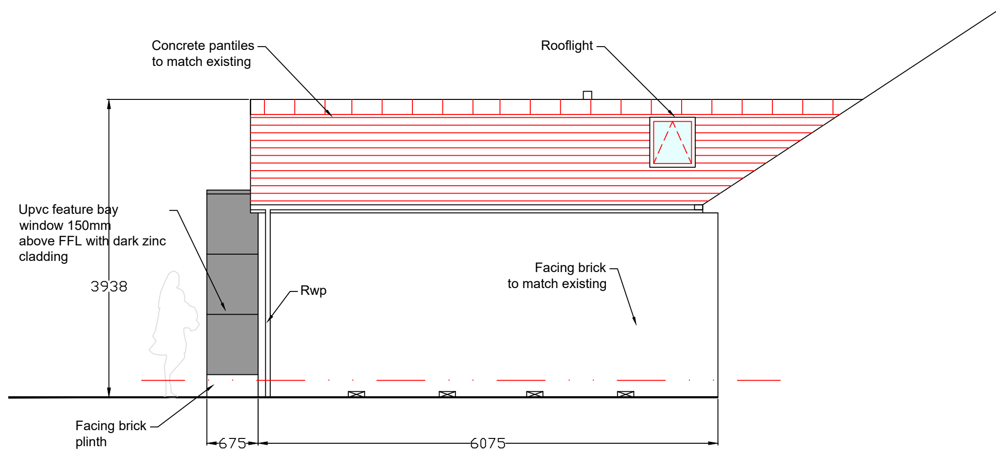
PROPOSED SIDE ELEVATION TO REAR 1:50
