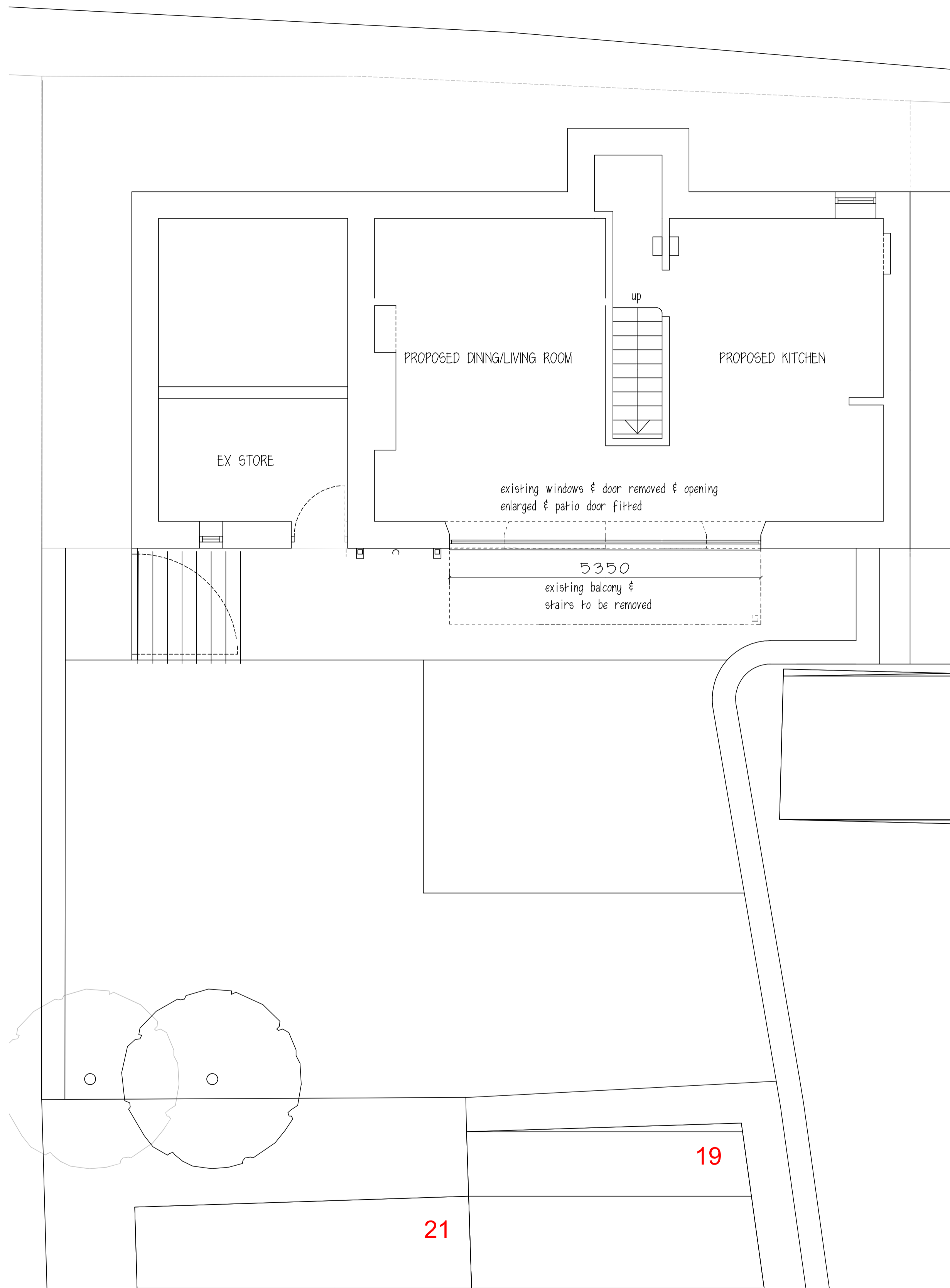
Lower Ground Floor Plan
