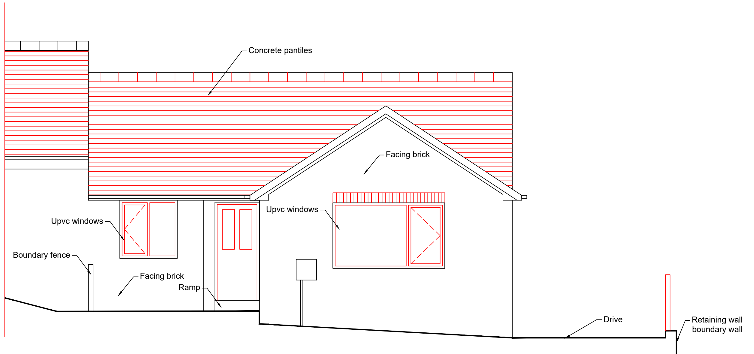
EXISTING FRONT ELEVATION 1:50
