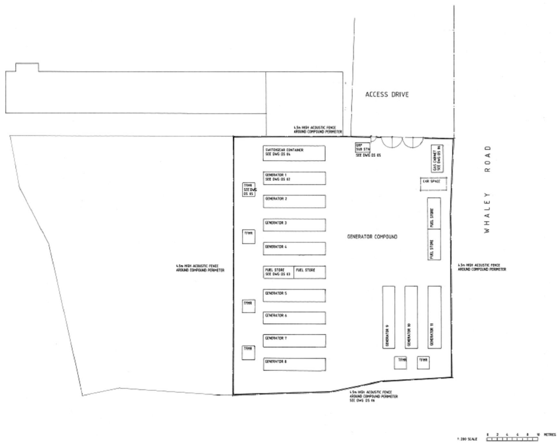
Figure 2 - Proposed Compound Arrangement
