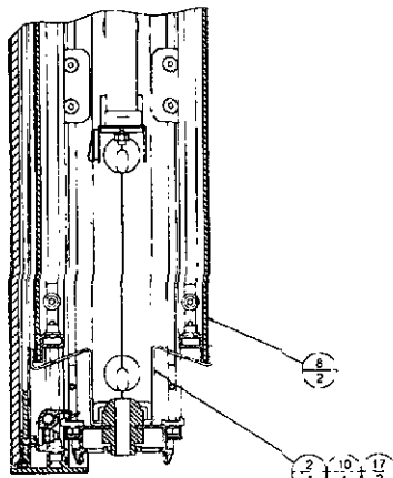
DETAIL A SCALE 0.50
