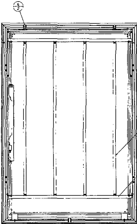
SECTION X-X
