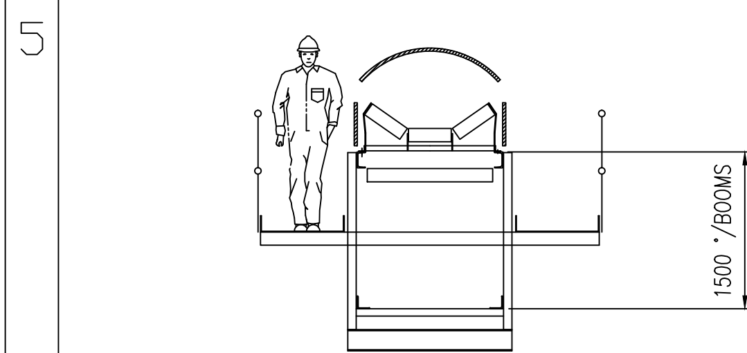
TYPICAL CONVEYOR GANTRY SECTION
