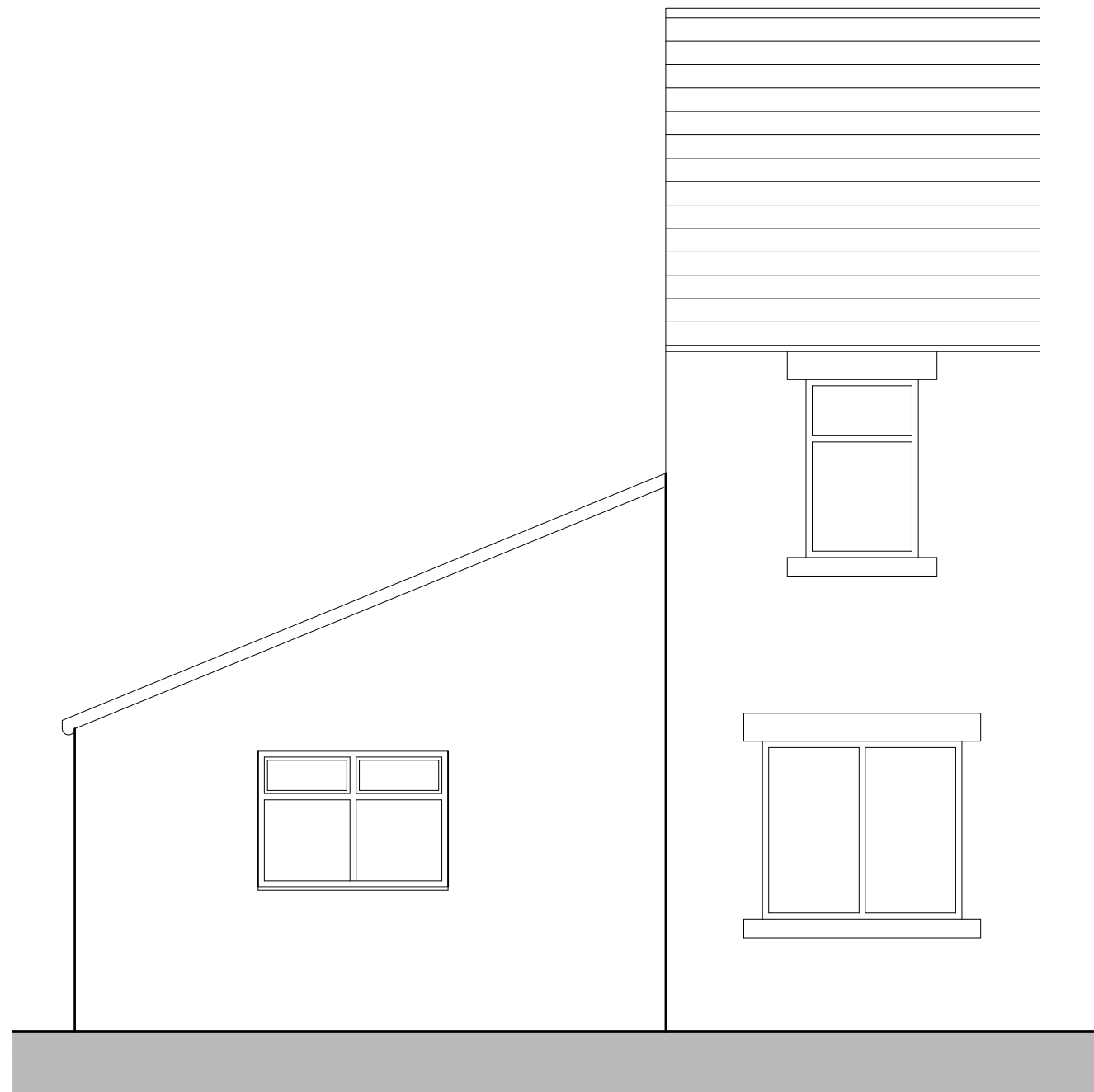
Existing Front Elevation 1:50
