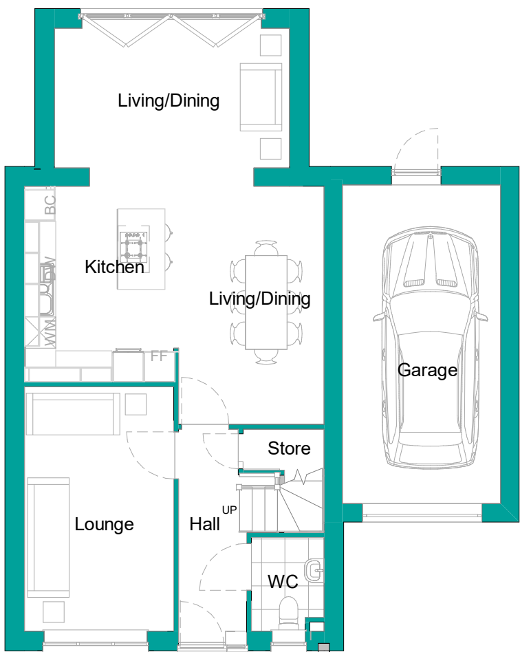
Ground Floor. 1 : 100
