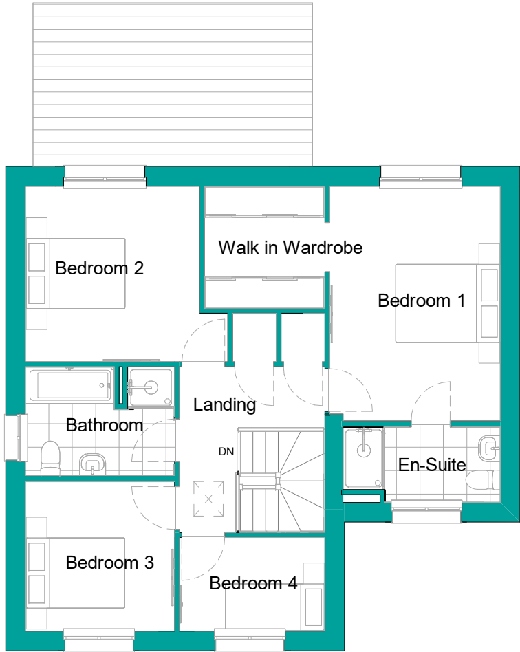
First Floor. 1 : 100
