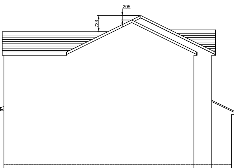
LEFT ELEVATION - PROPOSED
