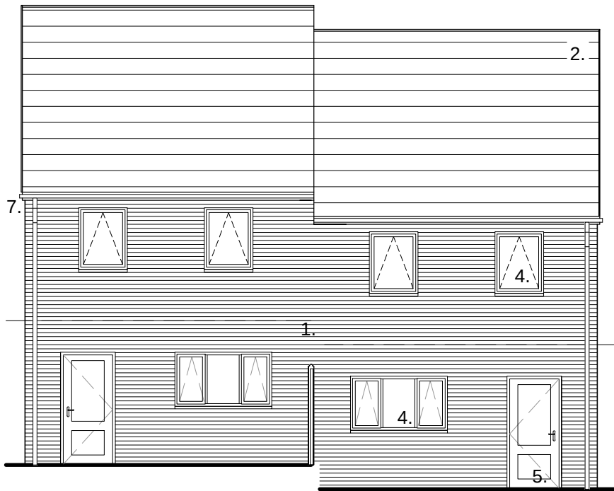
Rear Elevation
