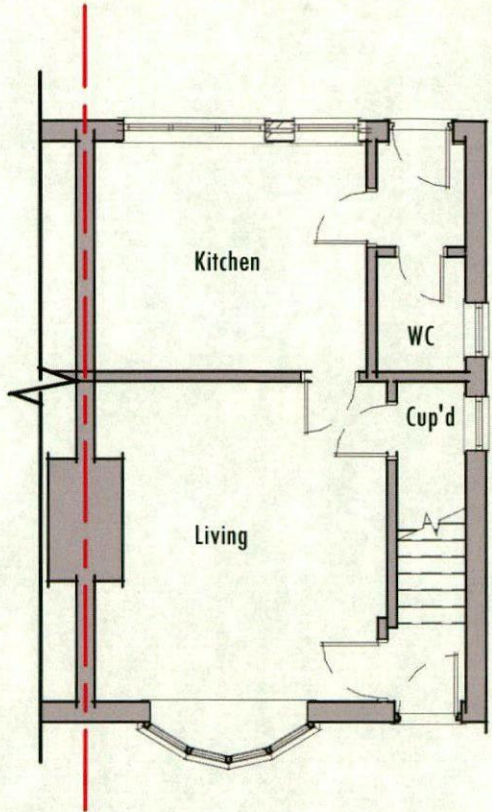
Ground Floor 1 : 100
