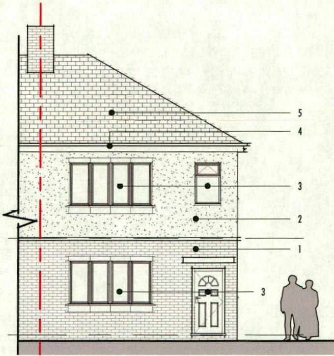
Front Elevation 1 : 100
