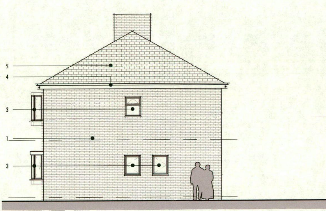
Side Elevation 1 : 100
