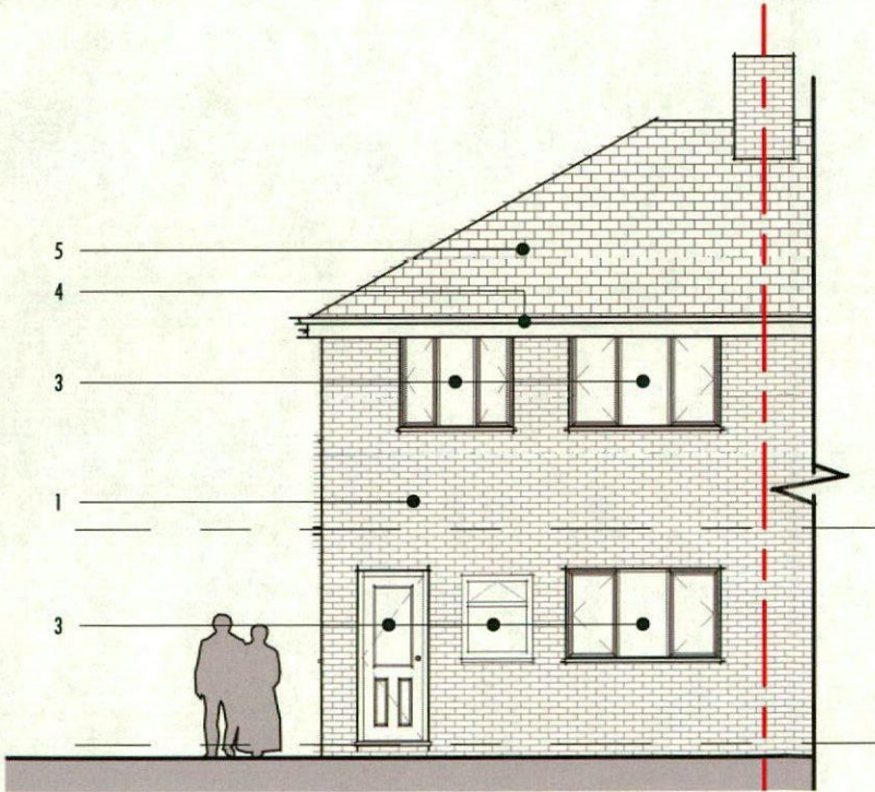
Rear Elevation 1 : 100
