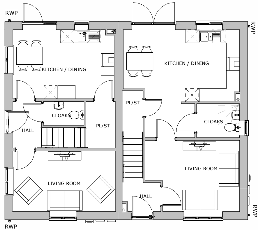
Ground Floor 1 : 100
