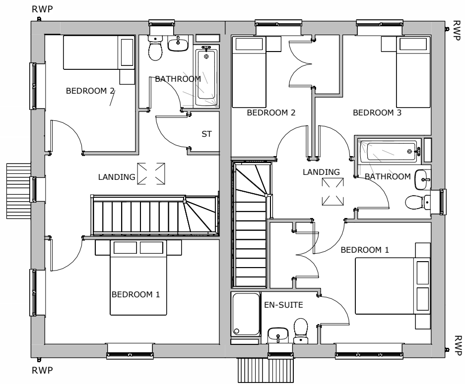
First Floor 1 : 100
